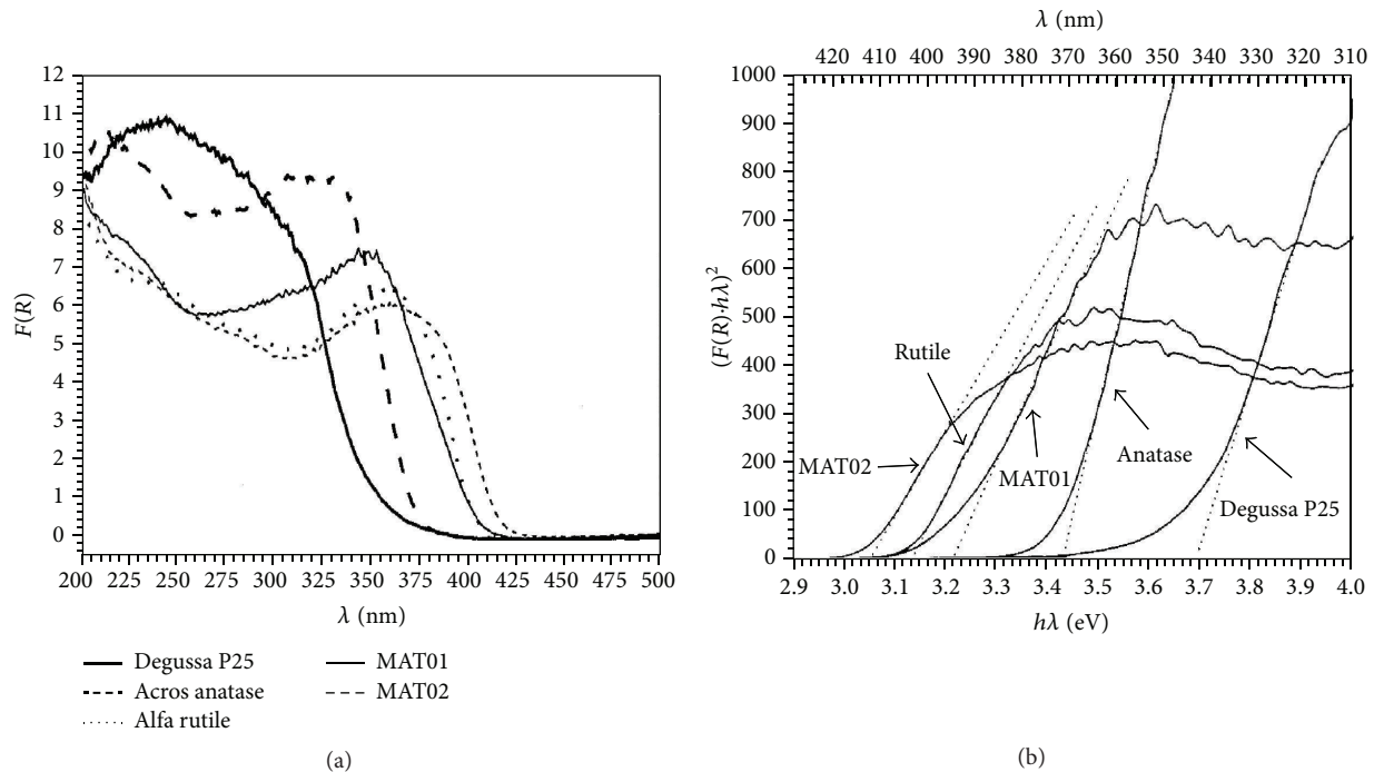
FIGURE 17: (a) UV-Vis DRS spectra of the mixed oxide materials MAT01, MAT02 along with Degussa P25, Acros anatase, and Alfa rutile materials and (b) the corresponding Kubelka-Munk function plot (reprinted with permission from [87]).
