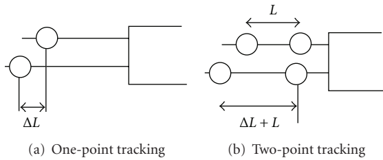
FIGURE 6: Strain methods.
