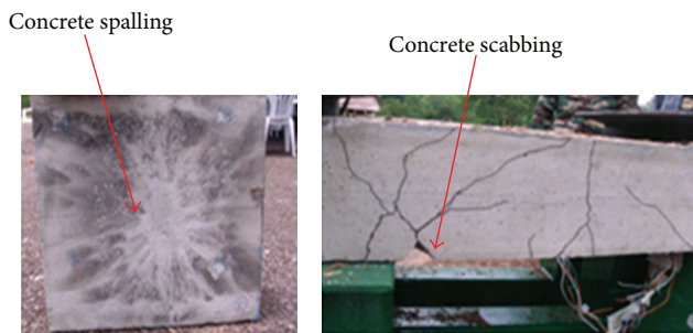
FIGURE 7: Failure mode of NRC panel subjected to blast loading.
