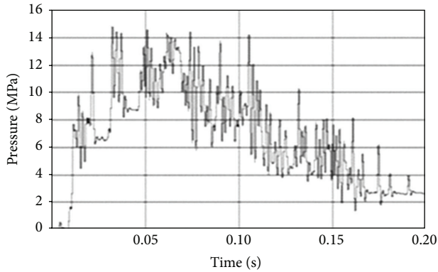
FIGURE 9: Peak overpressure resulted from 1 kg of plastic explosive at a distance of 300 mm.
