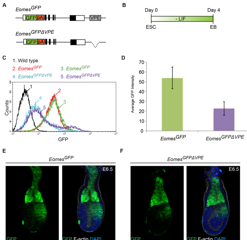
Fig. 3. VPE deletion profoundly reduces the level of Eomes GFP reporter expression. (A) Configuration of the Eomes GFP and Eomes GFP \Delta VPE alleles (Fig. S5). (B) Schematic of the embryoid body (EB) differentiation protocol. (C, D) Flow cytometry analysis of wild-type, Eomes GFP/+ and Eomes GFP \Delta VPE/+ day 4 EBs. (E, F) Confocal images of Eomes GFP and Eomes GFP \Delta VPE reporter expression in E6.5 embryos stained with anti-GFP antibody, DAPI (DNA) and phalloidin (F-actin). Domains of reporter expression are not perturbed by VPE deletion.
