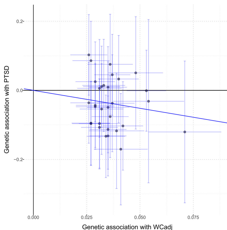
Fig. 1 SNP-exposure (WC adj associations) and SNP-outcome (PTSD associations) coefficients used in the MR analysis. Error bars (95% CIs) are reported for each association. The solid line represents the inverse-variance-weighted estimate
