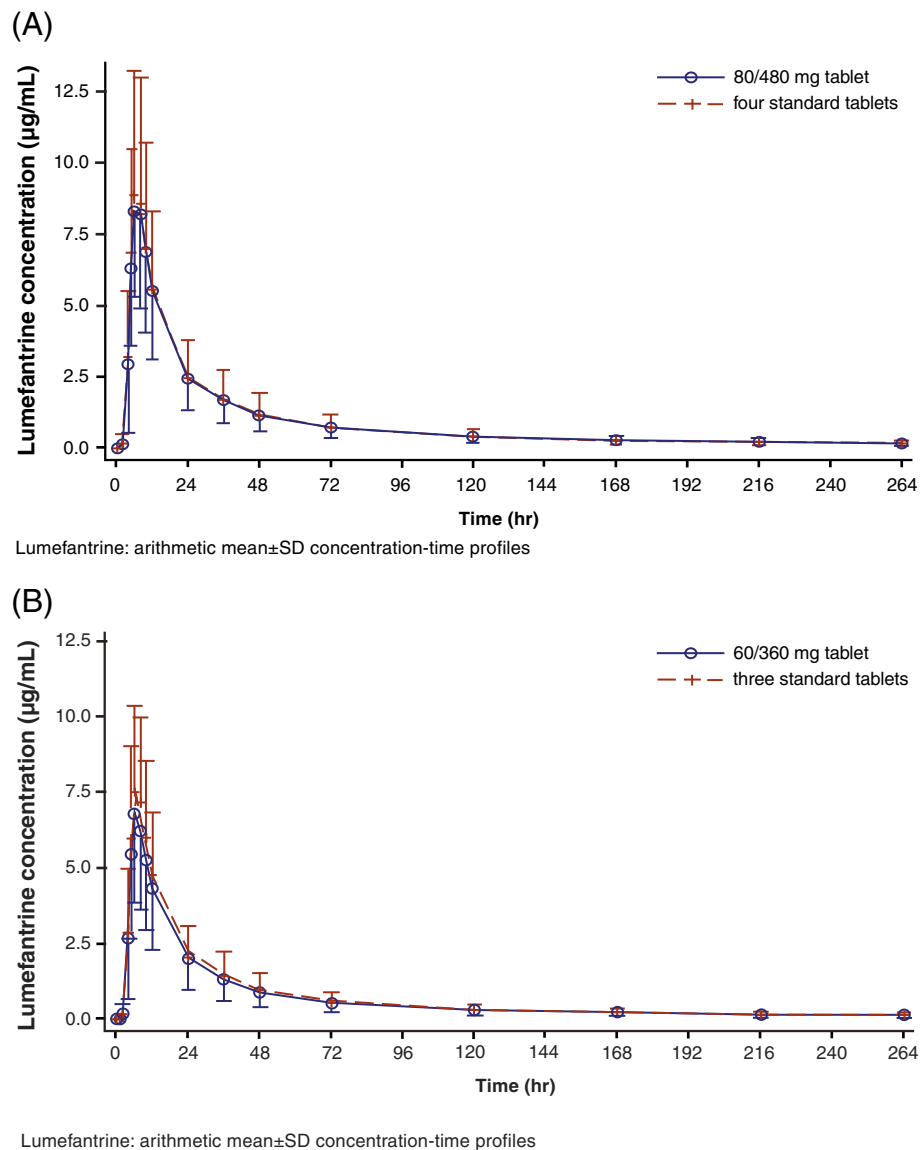
Figure 2 Lumefantrine: arithmetic mean ± SD concentration-time profiles. Mean plasma concentration-time profiles for comparison of (A) 80/480 mg tablet and four standard tablets (B) 60/360 mg tablet and three standard tablets.
