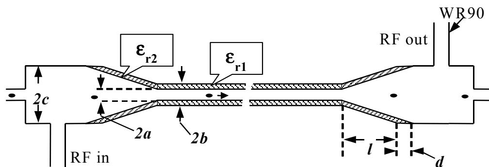
FIGURE 1. Example of an 11.424 GHz Structure of the new scheme.
