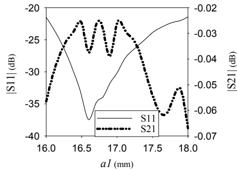
FIGURE 10. S parameters of single side coupler at 11.424GHz varying with al
