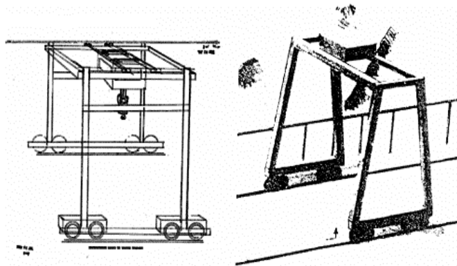
FIGURE 1. Above left is Pat Price’s drawing of his psychic impressions of a gantry crane at the secret Soviet research and development site at Semipalatinsk, showing remarkable similarity to a later CIA drawing based on satellite photography shown at right. Note, for example, that both cranes have eight wheels.
