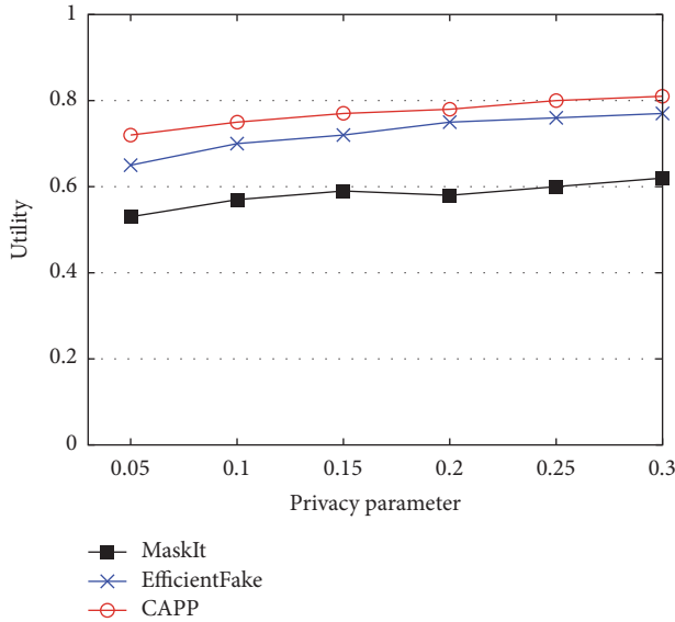
FIGURE 4: Privacy-utility tradeoff (home as sensitive).
