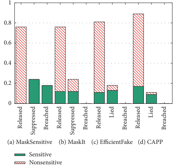
FIGURE 2: Privacy breach comparison (home as sensitive).
