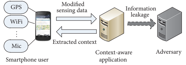
FIGURE 1: A mobile phone context sensing system [7, 8].
