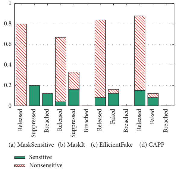
FIGURE 3: Privacy breach comparison (random as sensitive).
