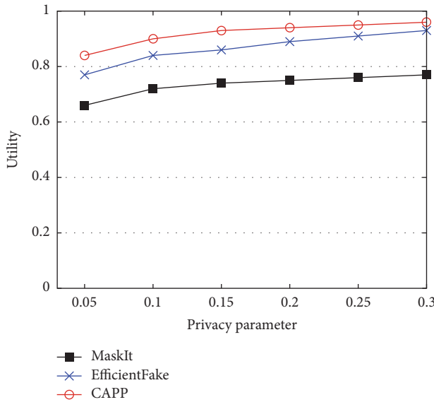
FIGURE 5: Privacy-utility tradeoff (random as sensitive).
