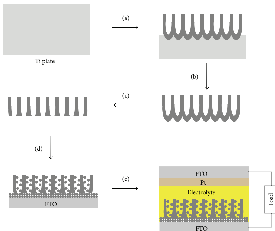
FIGURE 10: Scheme for fabricating a DSSC based on a \text{TiO}_2 nanotube membrane filled with \text{TiO}_2 nanoparticles: (a) 1st anodization, then annealing, (b) 2nd anodization and detachment of \text{TiO}_2 film, (c) ion milling, (d) filling \text{TiO}_2 nanoparticles, attaching on fluorine-doped thin oxide (FTO) glass, treating with \text{TiCl}_4 , and then annealing in air, and (e) dye adsorption and fabrication of a DSSC. Reprinted with permission from [48]. Copyright 2011, Elsevier.
