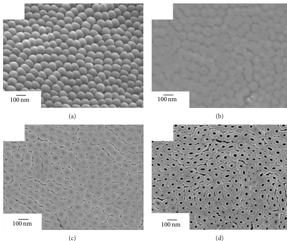
FIGURE 7: SEM images taken by Rho et al. of the freestanding \text{TiO}_2 films after ion milling of (a) 0, (b) 20, (c) 30, and (d) 90 minutes. Reprinted with permission from [45]. Copyright 2012, American Chemical Society.
