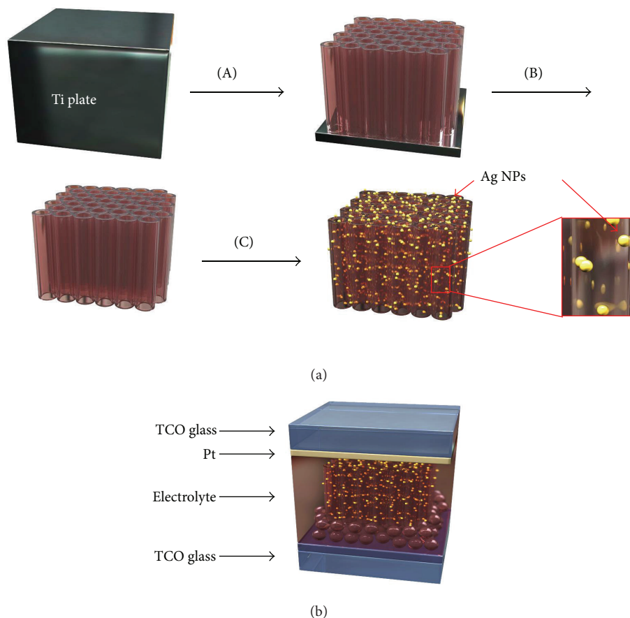
FIGURE 9: (a) Schematic of plasmon DSSC based on method reported by Rho et al. (A) Ti anodization in organic electrolyte, (B) freestanding TiO 2 nanotube arrays, (C) formation of Ag nanoparticles on TiO 2 nanotube arrays by UV irradiation at 254 nm. (b) Schematic of an assembled cell. Reprinted with permission from [47]. Copyright 2014, Elsevier.
