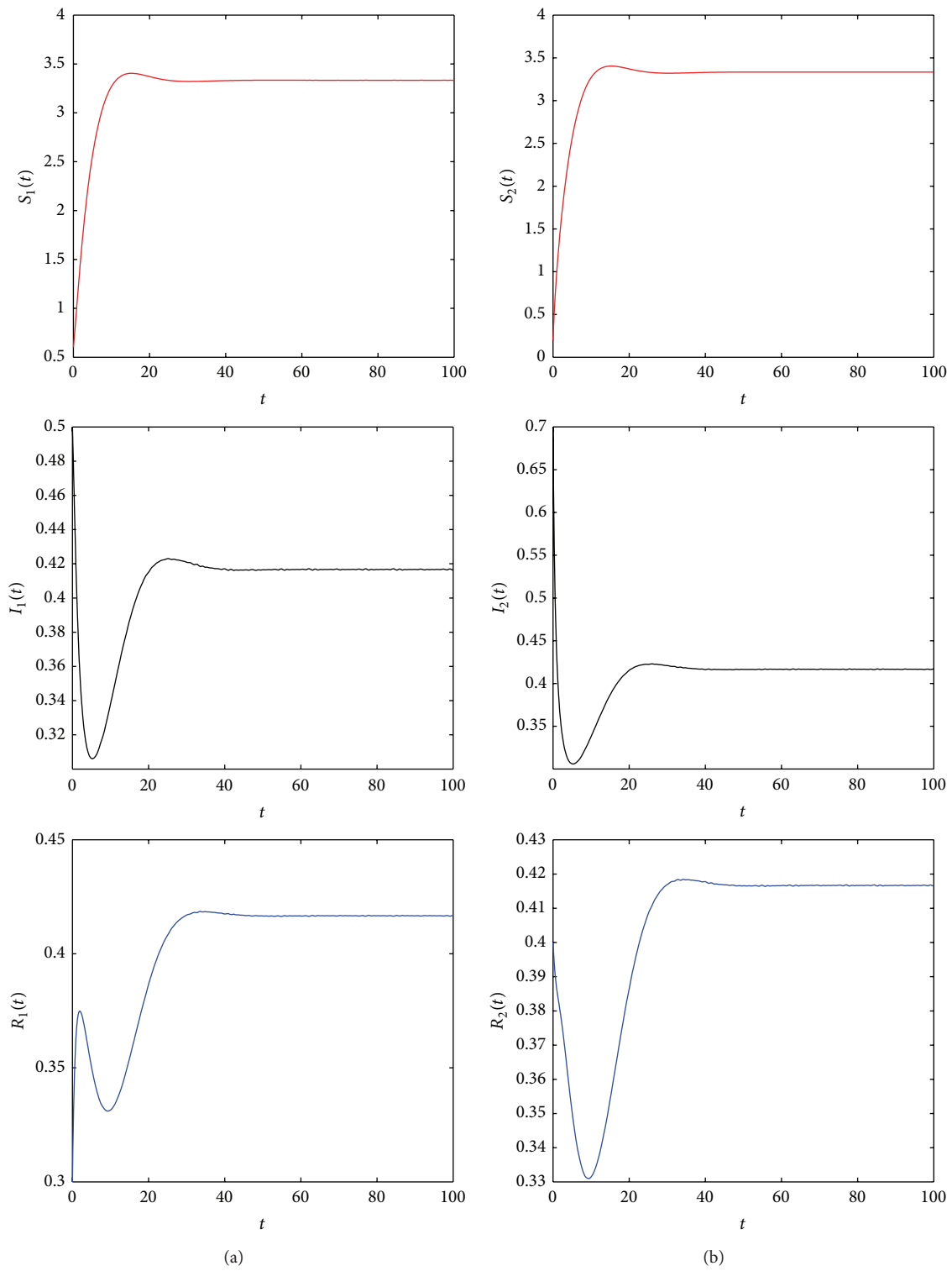
FIGURE 2: (a) shows movement paths of S_1, I_1 , and R_1 as functions of time t . (b) shows movement paths of S_2, I_2 , and R_2 as functions of time t . Here a = 1, b = 0.2, c = 0.4, d = 0.2, \alpha = 0.8, \beta = 0.6 , and \gamma = 0.5 . Initial data are 0.6, 0.5, 0.3, 0.2, 0.7, 0.4.
