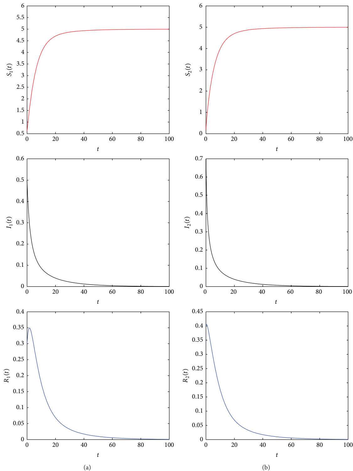
FIGURE 1: (a) shows movement paths of S_1 , I_1 , and R_1 as functions of time t . (b) shows movement paths of S_2 , I_2 , and R_2 as functions of time t . Here a = 1 , b = 0.2 , c = 0.4 , d = 0.2 , \alpha = 0.3 , \beta = 0.6 , and \gamma = 0.5 . Initial data are 0.6, 0.5, 0.3, 0.2, 0.7, 0.4.
