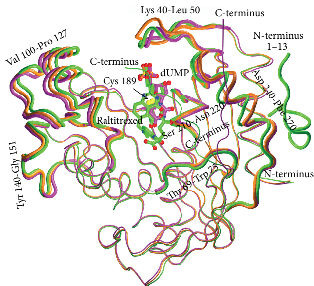
FIGURE 7: Superimposition of the main chains of the three structures: ligand-free mTS (orange, PDB ID: 3IHI), mTS-dUMP complex (violet, PDB ID: 4E5O), and mTS-dUMP-Raltitrexed complex (green, PDB ID: 4EB4). Ligands, dUMP and Raltitrexed, and catalytic Cys189 are shown as sticks. N, O, and S atoms are colored blue, red, and yellow, respectively. C atoms are colored the same as the corresponding tubes representing the main chains of respective complexes. The most differing main chain fragments are shown as thicker tubes. The 13-residue N-terminal fragment (1–13) in the tertiary complex, having no equivalents in the ligand-free enzyme and the binary complex, is also shown.
