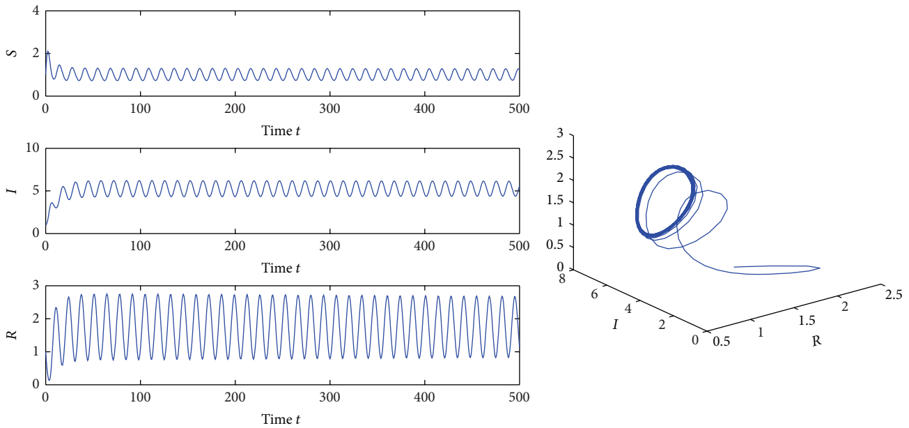
FIGURE 3: Behavior and phase portrait of system (2) with \tau_1 = 0, \tau_2 = 5 . Hopf bifurcation occurs from the virus infection equilibrium.
