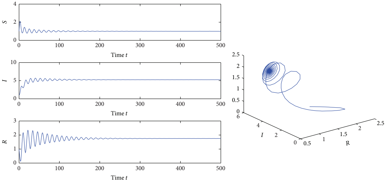
FIGURE 2: Behavior and phase portrait of system (2) with \tau_1 = 0, \tau_2 = 4 . The virus infection equilibrium is asymptotically stable.
