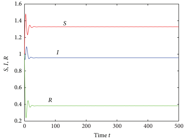
FIGURE 4: Numerical simulations of system (2) with parameter values: b = 0.8 , \beta = 0.4 , \mu = 0.3 , \gamma = 0.2 , and \nu = 0.2 , and E^* is globally asymptotically stable.
