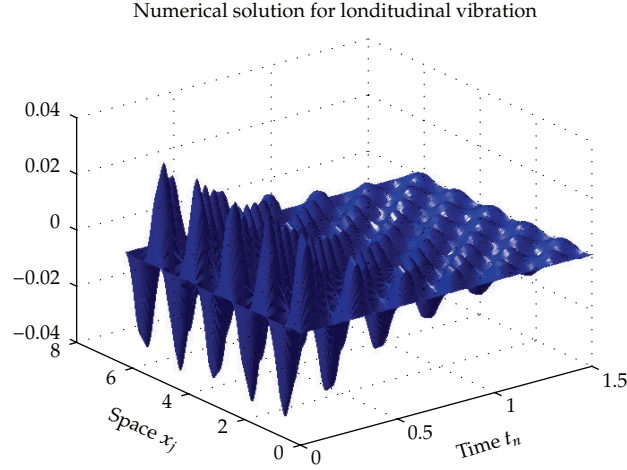
Figure 11: Total dissipation, \mu = 10 .
