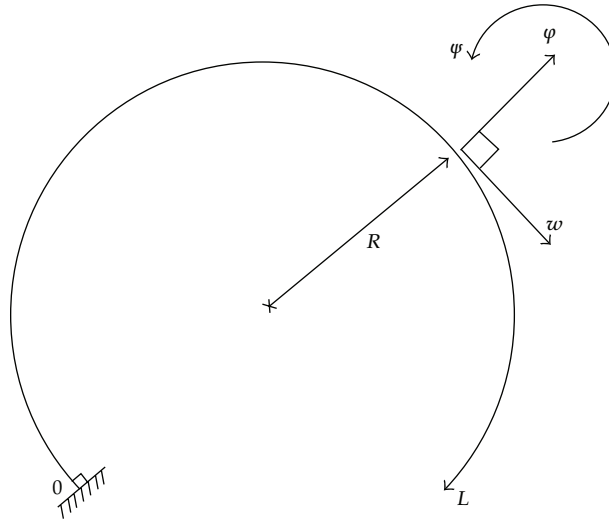
Figure 1: The circular arch.
