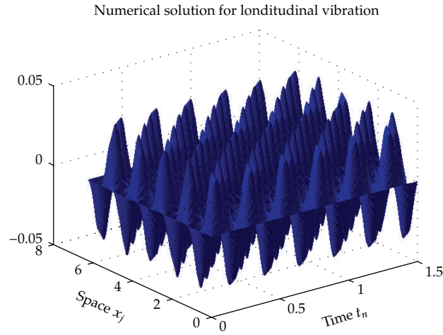
Figure 9: Conservative case, \mu = 10 .
