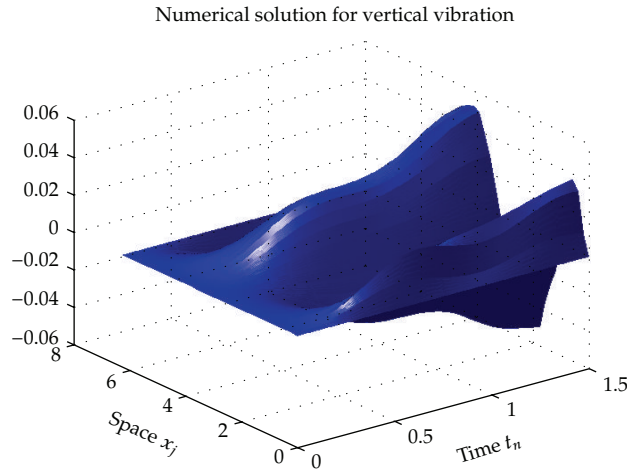
Figure 2: Conservative case, \mu = 3 .
