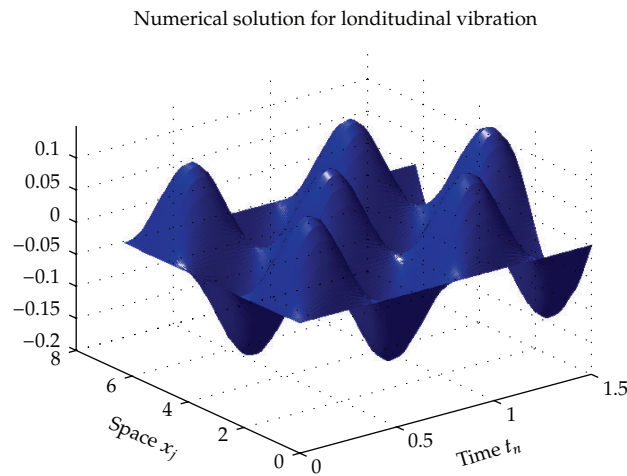
Figure 3: Conservative case, \mu = 3 .
