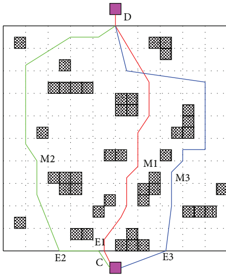
FIGURE 6: The path planning results in the complex environment.
