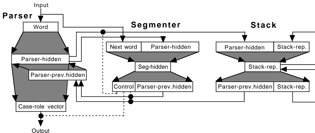
Figure 1: The SPEC sentence processing architecture. The system consists of the Parser (a simple recurrent network), the Stack (a RAAM network), and the Segementer (a feedforward network). The gray areas indicate propagation through weights, the solid lines stand for pattern transport, and the dashed lines represent control outputs (with gates). The lines controlling propagation within the Stack have been omitted.
