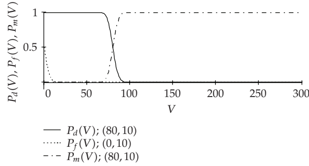
Figure 7: Intersection of three probability distributions: detection region.
