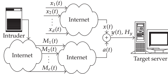
Figure 2: Illustration of abnormal traffic.
