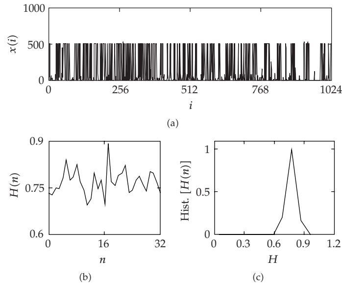
Figure 10: Verification of statistical invariable H . (a) A real-traffic time series; (b) estimate H(n) ; (c) histogram of H(n) .
