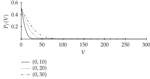
Figure 6: False alarm probability.
