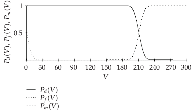
Figure 9: Case study: detection region.
