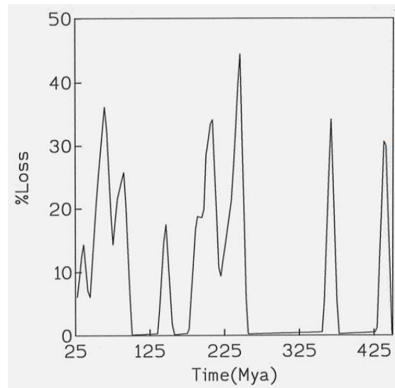
FIGURE 2. The percentage loss of species and genera for a number of major mass extinctions over the last 440 my vs. event time (mya) are shown as a peak-and-trough diagram. The data used are from Table 3.
