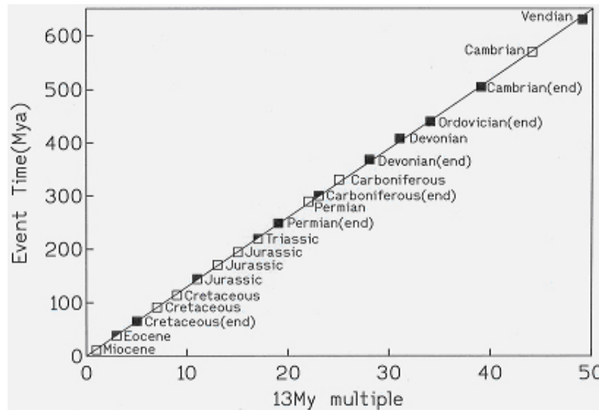
FIGURE 1. A linear plot of extinction event time (mya) vs. multiple of 13 my for mass extinctions over the Phanerozoic aeon. Major extinction events are shown in black whereas moderate ones are in black and white. The data used are from Table 1.
