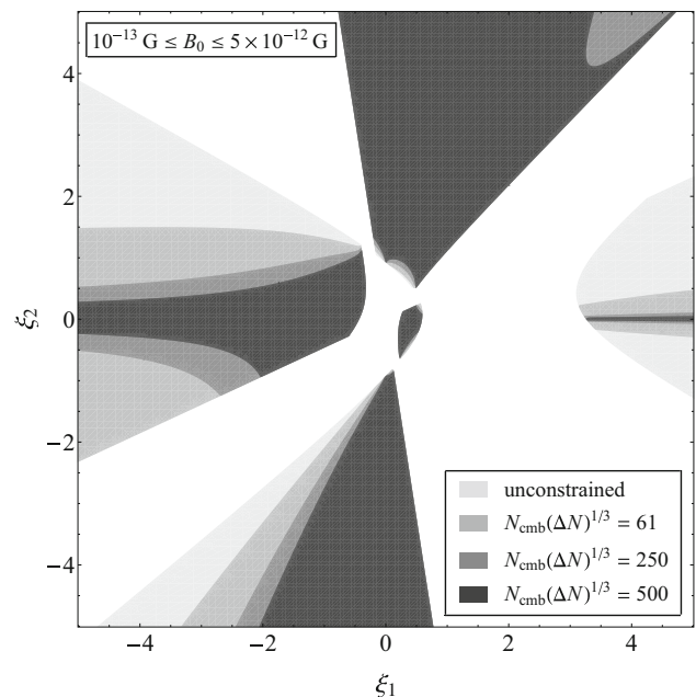
Fig. 3 Regions in the parameter space (\xi_1, \xi_2) , with \xi_1/\xi_2 \in \mathbb{X} [see Eq. (96)], where 10^{-13} \text{ G} \leq B_0 \leq 5 \times 10^{-12} \text{ G} and the electromagnetic back-reaction on inflation is completely negligible, with no constraints on curvature perturbations imposed ( light gray areas ). The dark gray regions represent the same regions after imposing the constraint (148) which assures that scalar curvature perturbations generated by the inflation-produced electromagnetic field are compatible with CMB observations [the darkness increases as (N_{cmb}/61)(\Delta N)^{1/3} increases]
