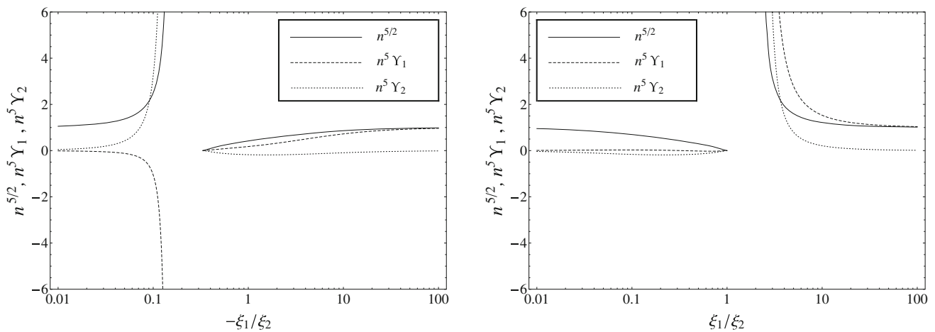
Fig. 1 The quantities n^{5/2} (continuous lines), n^5 \Upsilon_1 (dashed lines), and n^5 \Upsilon_2 (dotted lines) [which appear in Eqs. (114), (115), and (116), respectively], as a function of \xi_1/\xi_2
