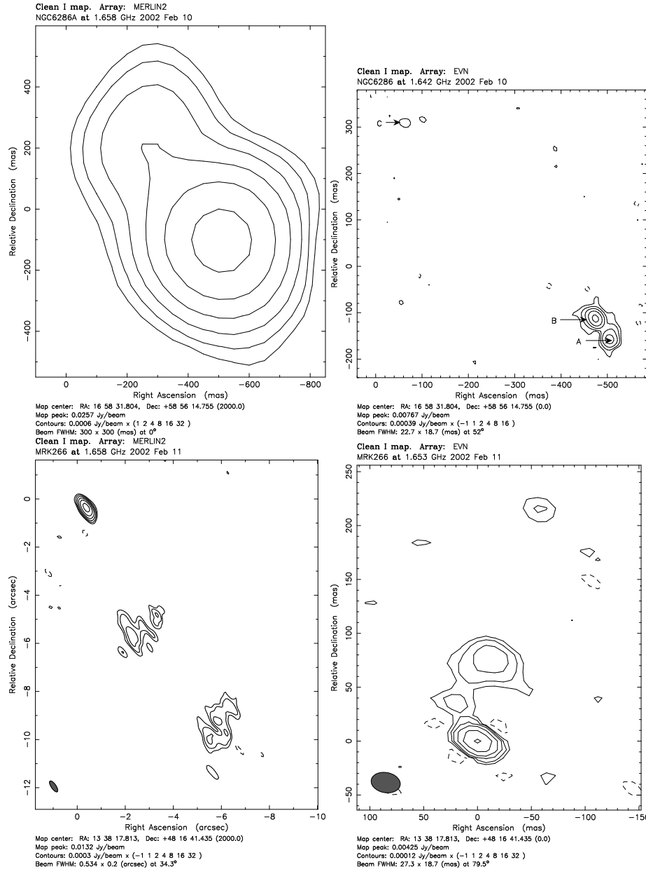
Fig. 2. Top Left: The MERLIN image of NGC6286 with a restoring beam of 300 mas. The peak is 25.7 mJy/bm and the contours are drawn at 1,2,4,8,16,32 x 0.6 mJy/bm. Top Right: The EVN image of NGC6286 restored with a beam of 22.7x18.77 mas. The peak is 7.6 mJy/bm and the contours are drawn at 1,2,4,8,16 x 0.39mJy/bm. Bottom Left: The MERLIN image of Mrk 266 with a restoring beam of 534x200 mas. The peak is 13.2 mJy/bm and the contours are drawn at 1,2,4,8,16,32 x 0.3 mJy/bm. Bottom right: The EVN image of Mrk 266 restored with a beam of 27x18 mas. The peak is 4.2 mJy/bm and the contours are drawn at 1,2,4,8,16 x 0.12mJy/bm.
