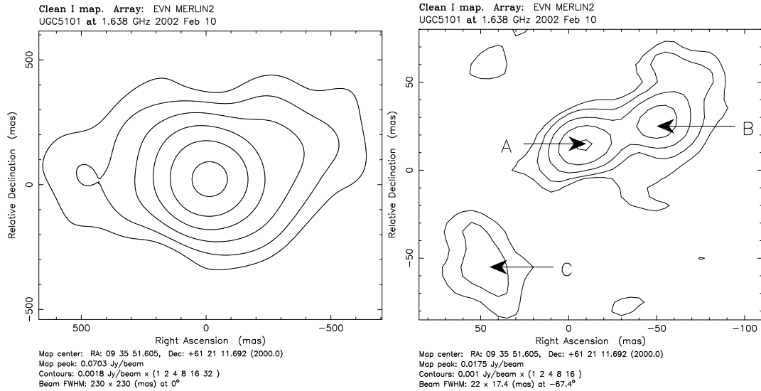
Fig. 1. Left: The MERLIN image of UGC 05101 with a restoring beam of 230 mas. The peak is 70.3 mJy/bm and the contours are drawn at 1,2,4,8,16,32 x 1.8 mJy/bm. Right: The EVN image of UGC 05101 restored with a beam of 22x17.4 mas. The peak is 17.5 mJy/bm and the contours are drawn at 1,2,4,8,16 x 1mJy/bm.
