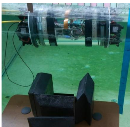
Figure 9 Submerged ROV gamma detector experiments. Cs source was placed up against the edge of the tank with the AVEXIS parallel to the source submerged.
