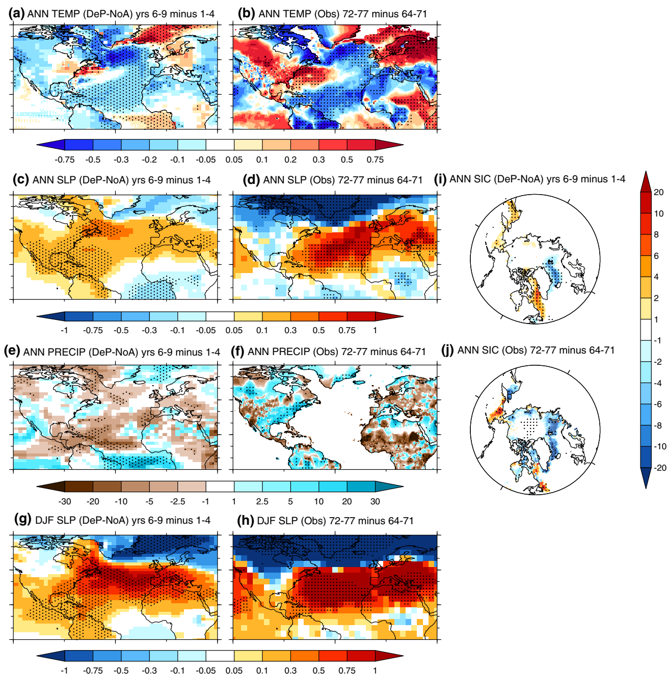
Fig. 9 shows the predicted and observed surface climate impact of 1960s cooling. a shows the difference between years 6–9 minus years 1–4 (i.e. the in-hindcast trend) of annual mean SAT and SST [°C] for the DePreSys hindcasts initialised between 1963–1968, relative to the same difference in NoAssim (i.e. \Delta DeP - \Delta NoA , see text for details). b the difference between 1972–1977 and 1964–1971 for observations
