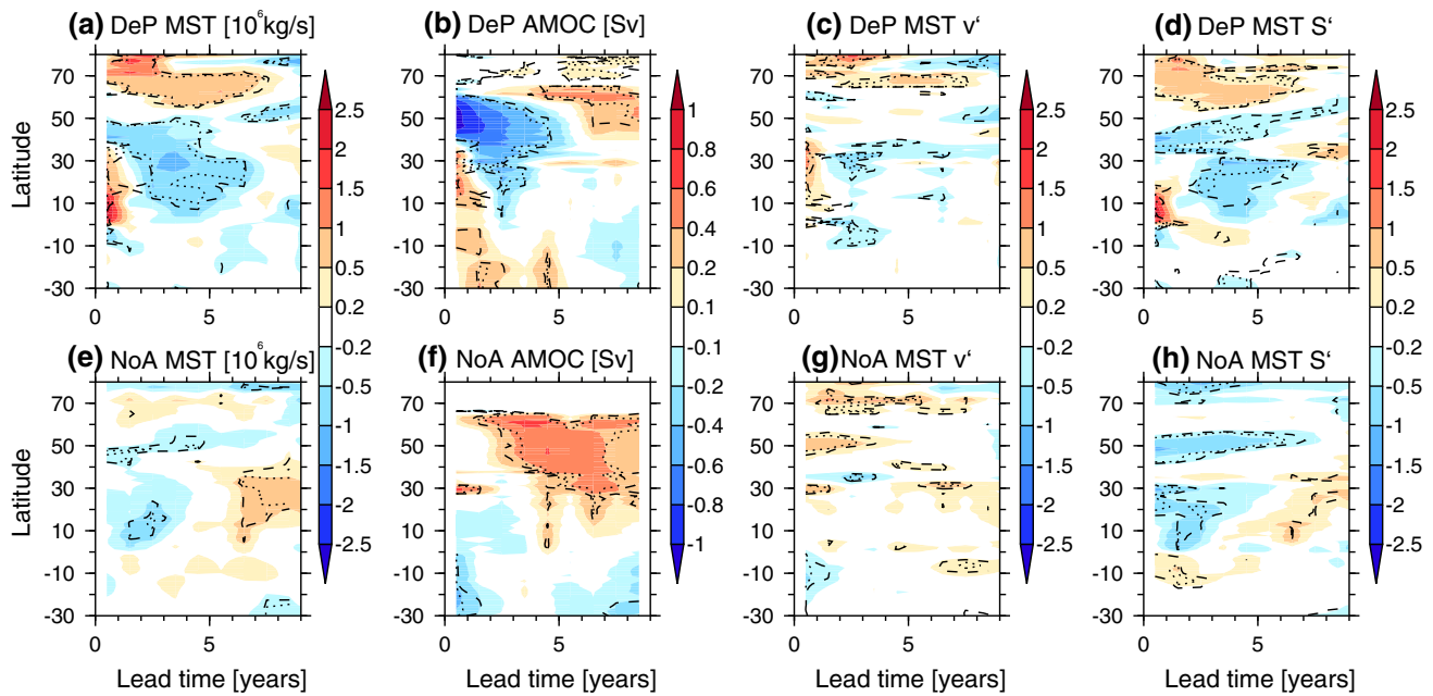
Fig. 8 latitude-time plots of anomalous ocean salt transports and overturning. a The anomalous meridional salt transport (MST) [ 10^6 \text{ kg s}^{-1} ] averaged over DePreSys hindcasts started between 1963 and 1968, relative to climatology defined as the mean over year 1 from all NoAssim hindcasts (1960–2005). b as a but for the AMOC [Sv]. c and d are as a but for the contribution to the transport which is due
