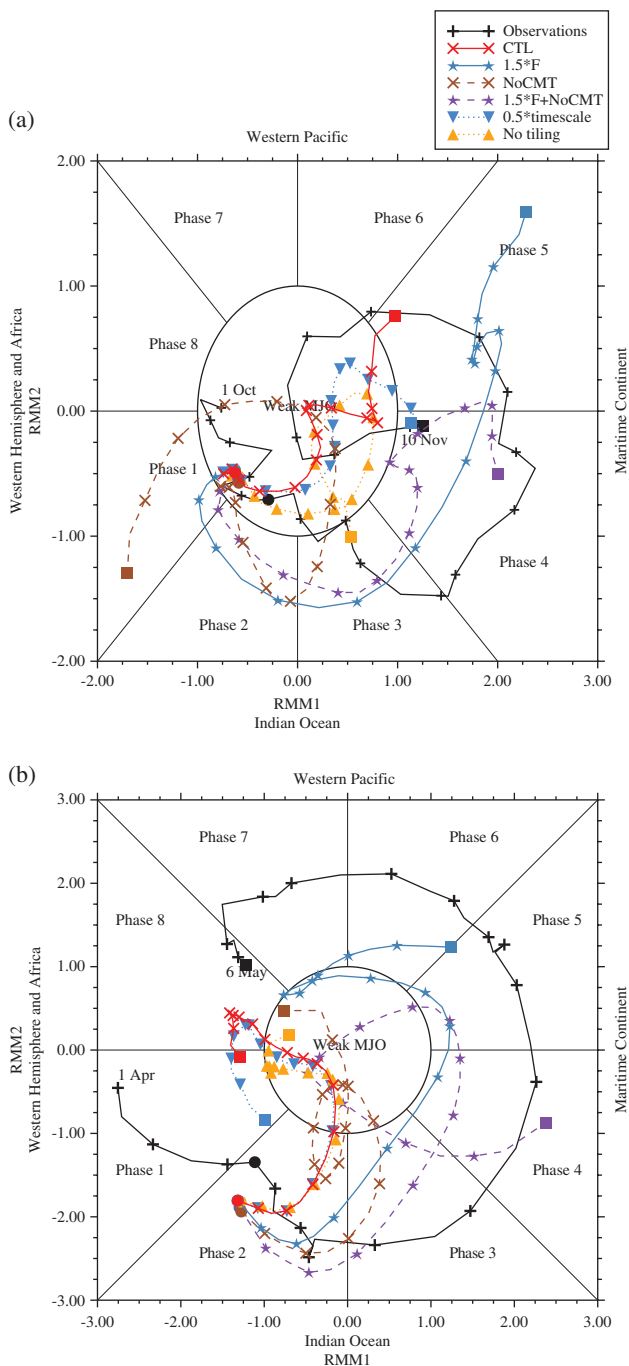
Figure 2. For (a) Oct08 and (b) Apr09 cases, time series of RMM indices from observations (black line) and the hindcast sets shown in the key at the top right (other colours). Day 1 (30) is marked with a circle (square); symbols are spaced every 2 days along the traces.
