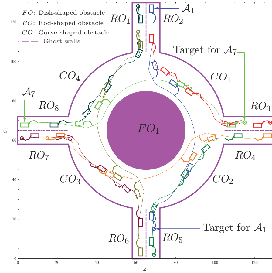
Fig. 7. Scenario 1. The resulting trajectories of the 3DNMs with dimensions \ell_0 = 1.5 , b_0 = 0.7 and \ell_1 = \ell_2 = \ell_3 = 0.7 . Also, \rho_{i0} = 1 , \rho_{ik} = 1 ( k = 1, 2, 3 ), \delta_{ij} = 200 , j = 1, \dots, 4 , the initial velocities are v_i(0) = 3 , \omega_{i0}(0) = 0.2 , and \omega_{i1}(0) = \omega_{i2}(0) = 0.05 , for i = 1, \dots, 8 .
