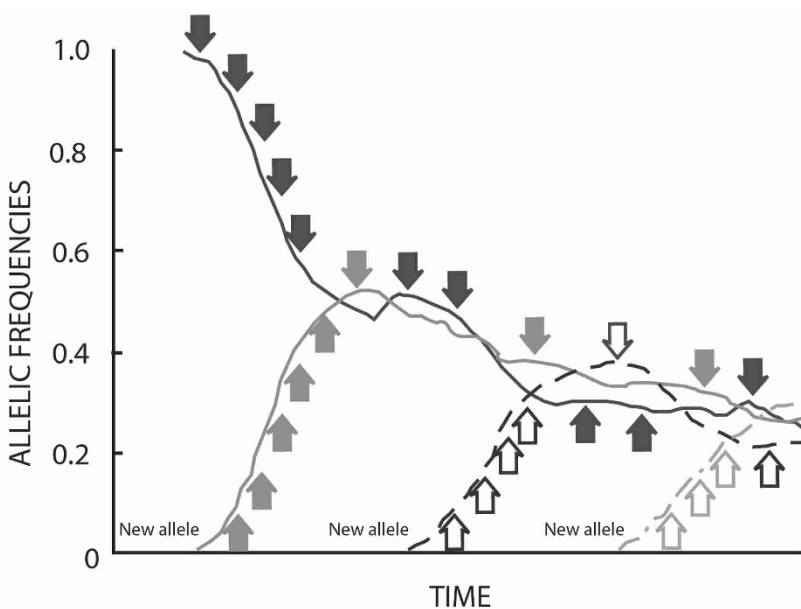
Figure 4. A theoretical graph of the MHC allelic turnover at the host population level to control the pathogen variability and its escapement mechanisms (source Apanius et al. [3]).
