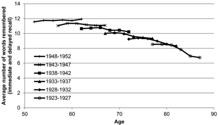
Figure 2. Immediate and delayed word recall by cohort and age. Notes: Sample is the balanced panel who responded to all six waves of ELSA. Sample size = 4,584. Source: Authors’ calculations using waves 1–6 (2002–03 to 2012–13) of the ELSA.
