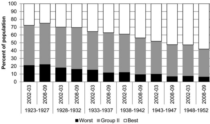
Figure 1. Numerical ability in 2002–03 and 2008–09 by cohort. Note: Sample size is 9,850 for wave 1 and 6,042 for wave 4. Sample is individuals who provide an answer to the numeracy questions in each wave. Source: Authors’ calculations using waves 1 and 4 of the ELSA.
