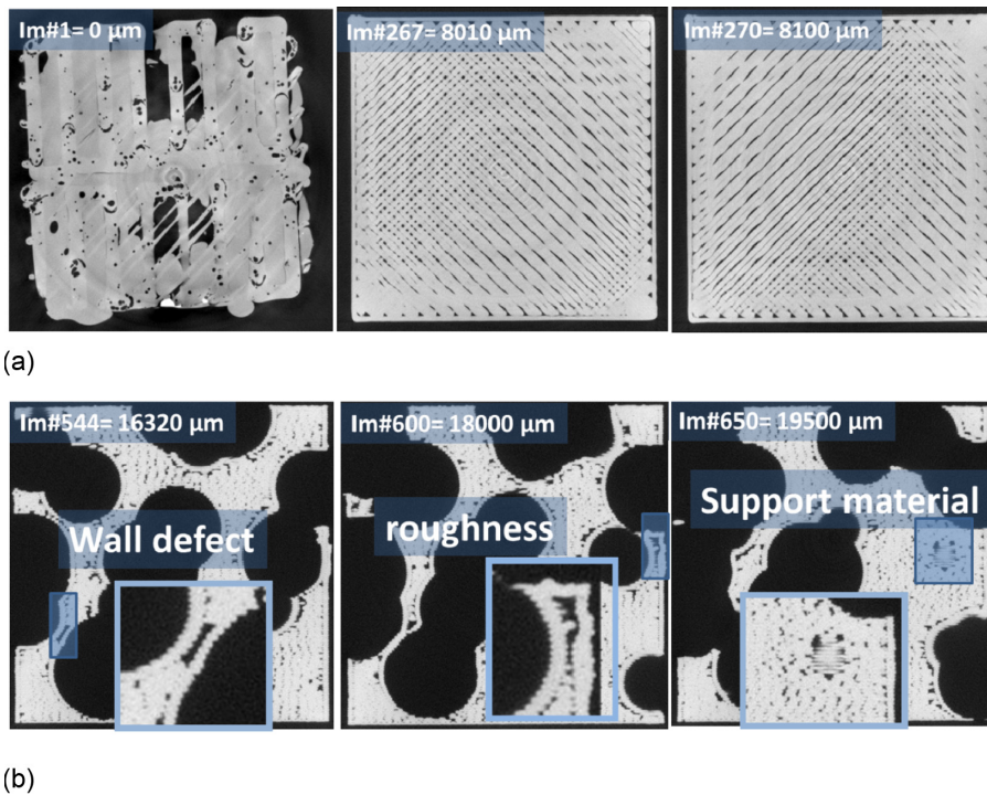
Figure 6. Microstructural defects in ABS polymer printed using FDM. Analysis is performed using X-ray micro-tomography. Two examples are shown one is (a) a dense ABS block and the other is (b) airy ABS materials exhibiting more than 60% of porosity.
