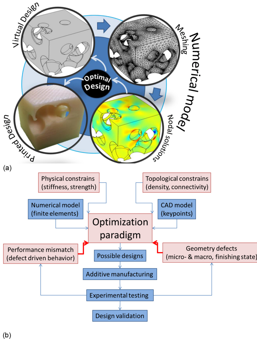
Figure 5. (a) Classical view of topological optimisation, (b) Modified scheme with defect sensitive topology optimisation of AM.
