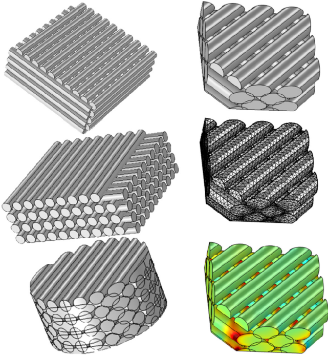
Figure 7. Towards modelling of AM process.
