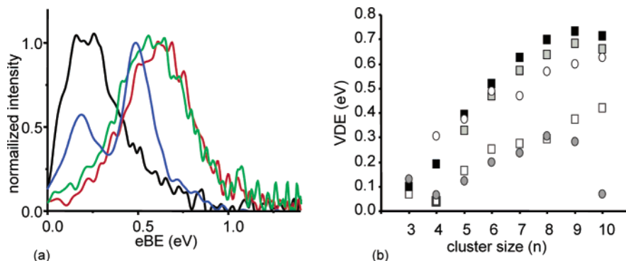
Figure 7. (a) Comparison of I^-(D_2O)_8 spectra at delay times corresponding to VDE_{min} (black line), VDE_{max} (red line), and VDE(\infty) (green line), as labeled in Figure 6, to the spectrum of bare (D_2O)_8^- (blue line). Normalized signal intensity is plotted as a function of electron binding energy (eBE). (b) Comparison of I^-(H_2O)_n VDE_{min} , VDE_{max} , and VDE(\infty) to the VDEs of the corresponding bare (H_2O)_n^- clusters. Circles represent the two water isomers. Open squares are VDE_{min} ; gray and black squares are VDE_{max} and VDE(\infty) , respectively, of iodide-water. The VDE for (H_2O)_4^- was taken from Shin et al., 40 and (H_2O)_3^- and the weaker binding isomer of (H_2O)_5^- are from Hammer et al. 41 Error bars are estimated at \pm 60-80 meV for I^-(water)_n , n = 9-10 , and at \pm 30 meV for all other clusters.
