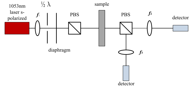
Figure 5. Schematic diagram of the experimental setup.
