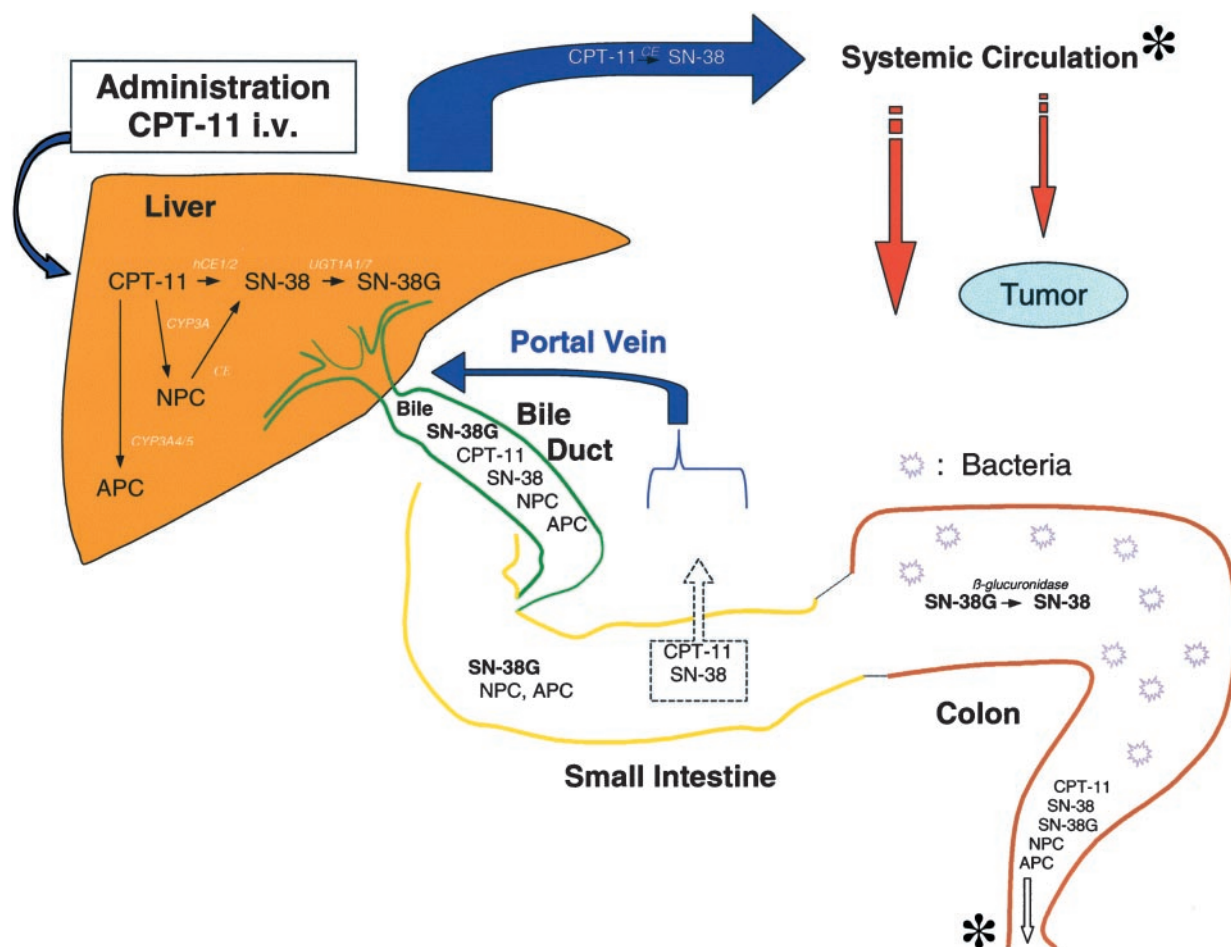
Fig. 1 Schematic representation of CPT-11 metabolism and enterohepatic recirculation. CE , carboxylesterase; hCE1/2 , human carboxylesterase isoforms 1 and 2; UGT1A1/7 , UDP glucuronosyltransferase isoforms 1A1 and 1A7; CYP3A4/5 , cytochrome P450 isoforms 3A4 and 3A5; APC , 7-ethyl-10-[4- N -(5-aminopentanoic acid)-1-piperidino]carbonyloxycamptothecin; NPC , 7-ethyl-10-[4- N -(1-piperidino)-1-amino]carbonyloxycamptothecin. * indicates the sites of drug measurement.
