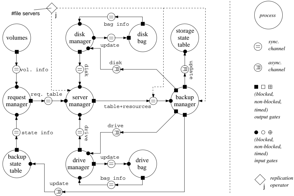
Figure 7: Global ADL structure diagram
