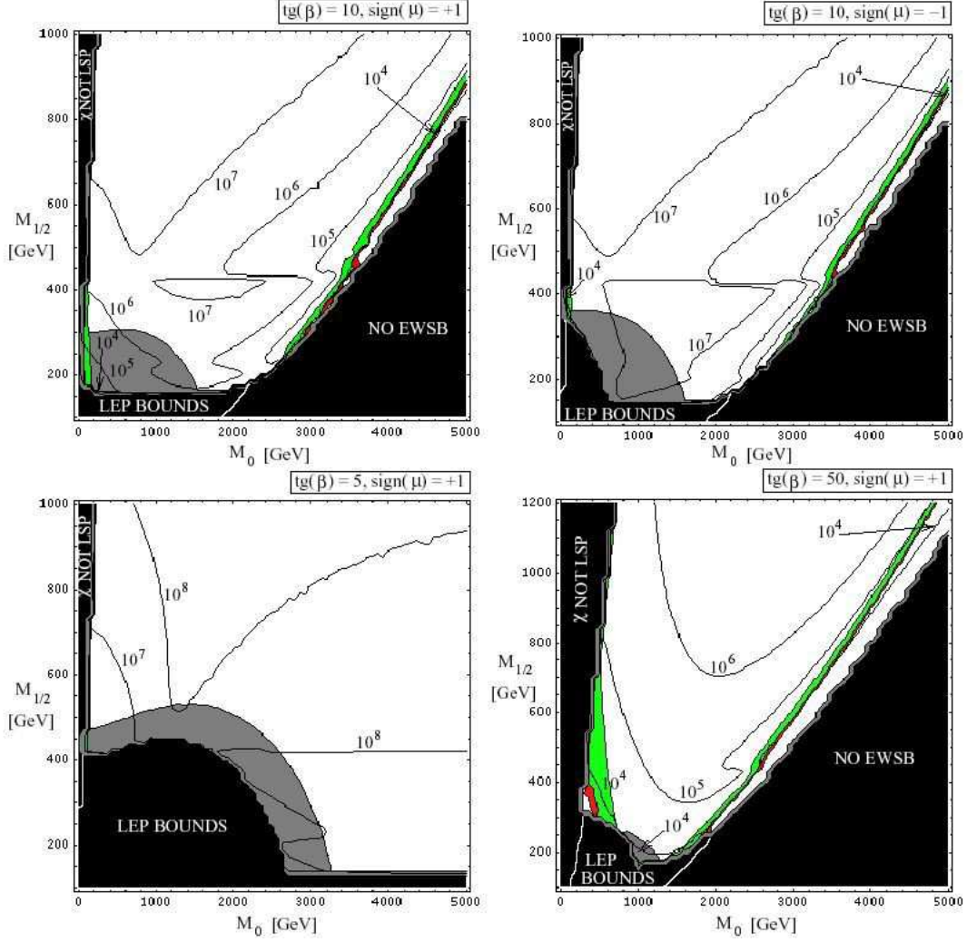
Fig. 9. Contour plots in the mSUGRA (m_0, m_{1/2}) plane, for the value of the normalization factor N_\chi , that allows the detection of the neutralino \gamma ray signal, with GLAST. In the green region 0.13 \leq \Omega_\chi h^2 \leq 0.3 , while the red region corresponds to the WMAP range 0.09 \leq \Omega_\chi h^2 \leq 0.13 [1]. The black region corresponds to models that are excluded either by incorrect EWSB, LEP bounds violations [46] or because the neutralino is not the LSP. In the dark shaded region m_{h_0} < 114.3 GeV [46], where h_0 is the lightest Higgs.
