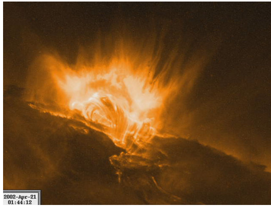
Fig. 3 Still from a movie: The flare SOL2002-04-21 observed in the Fe XII line at 195 Å (sensitive to 1.5 MK plasma) by the TRACE satellite. Note the different phases, starting with irregular brightening in the impulsive phase. The luminosity peaks when a sheet-like structures appears above the initial brightening. The diffuse emission at this time is attributed to the presence of the Fe XXIV (192 Å) line within the TRACE passband, emitted by a plasma of 20 MK. The flare proceeds into a long decay phase with post-flare loops growing in height (credit: TRACE Project, NASA)
