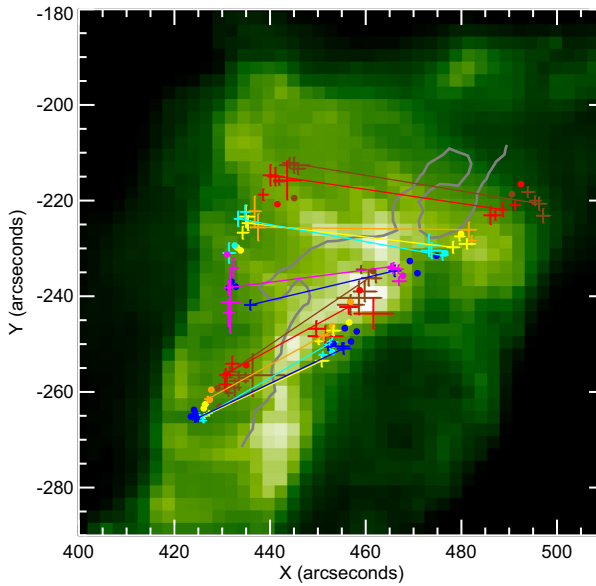
Fig. 8 Still from a movie: Hard X-ray footpoints (with error bars) observed with the RHESSI satellite during the flare SOL2002-11-09. Simultaneous footpoints are connected by a line colored sequentially with time. The footpoint information is overlaid on a SOHO/EIT image at 195 Å, indicating enhanced density in the corona. The movie shows two simultaneous footpoints connected by a vertical half-circle. The flux at each footpoint is indicated by the size of the purple circle at logarithmic scale (see Grigis and Benz 2005a). Movie courtesy of Paolo Grigis
