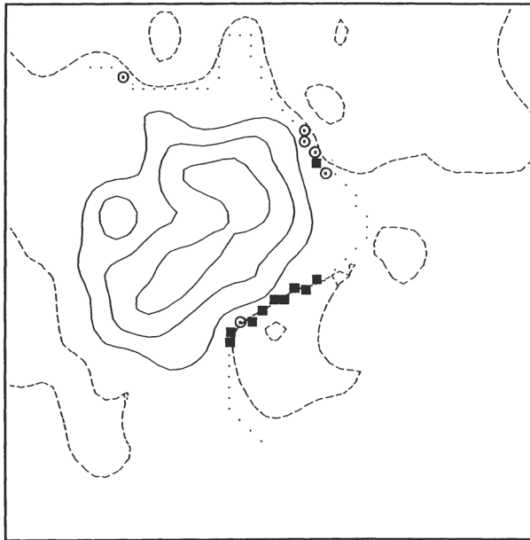
Fig. 6 Map of the line-of-sight magnetic field strength measured in a photospheric line by the MSFC magnetograph. Solid curves denote positive field, dashed curves the negative field, and the dotted curve the neutral line. Circles indicate where the transverse field deviates between 70^\circ and 80^\circ from the potential field (perpendicular to the neutral line), and filled squares indicate deviations >80^\circ . A large flare (X3 class) occurred several hours later at the location of the largest shear. Image reproduced with permission from Hagyard et al. (1990) , copyright by AAS
