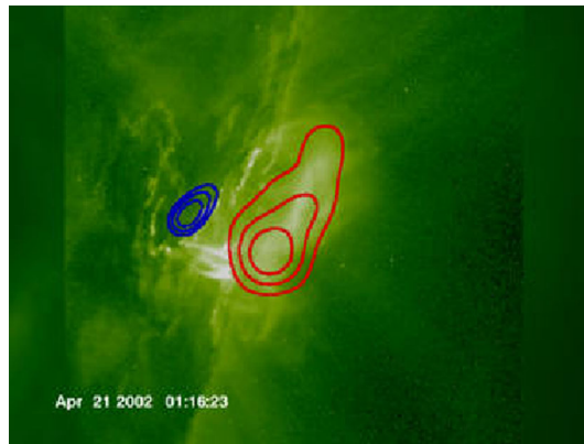
Fig. 4 Still from a movie: Zooming into the active region that hosted the major flare SOL2002-04-21. The movie starts in white light observed by the SOHO/MDI instrument, adds the coronal images observed by the SOHO/LASCO coronagraph, then changes to extreme ultraviolet observed by SOHO/EIT and later by the TRACE satellite, and later the RHESSI observations of the flare in soft X-rays ( red ) and hard X-rays ( blue ). The focus then goes to the associated coronal mass ejection observed by the coronagraph. The movie ends in a storm of streaks produced by energetic flare particles (mostly protons), hitting the detectors on the Solar and Heliospheric Observatory (SOHO) in space. Visualization by RHESSI scientists
