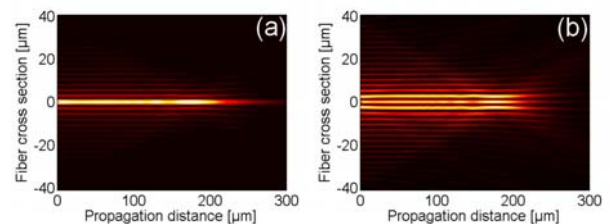
Fig. 3: (a) Free space propagation simulation of the ideal LP_{016} which has a propagation distance of 216 \mu\text{m} and (b) of the one found with the full vectorial mode solver which has a propagation distance of 218 \mu\text{m} .
