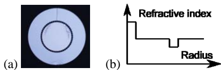
Fig. 1: (a): Microscope image of the fiber. The core is single-moded with a cutoff at 760 nm. The aircladding contains 60 holes. (b): Sketch of the refractive index profile of the investigated fiber.
