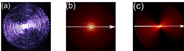
Fig. 2: a) Image of LP_{016} generated with a LPG in the aircladding fiber. The camera is slightly saturated to image the outer rings of the mode. b) An ideal LP_{016} generated with a scalar mode solver. c) One of two LP_{016} modes generated with a full vectorial mode solver.
