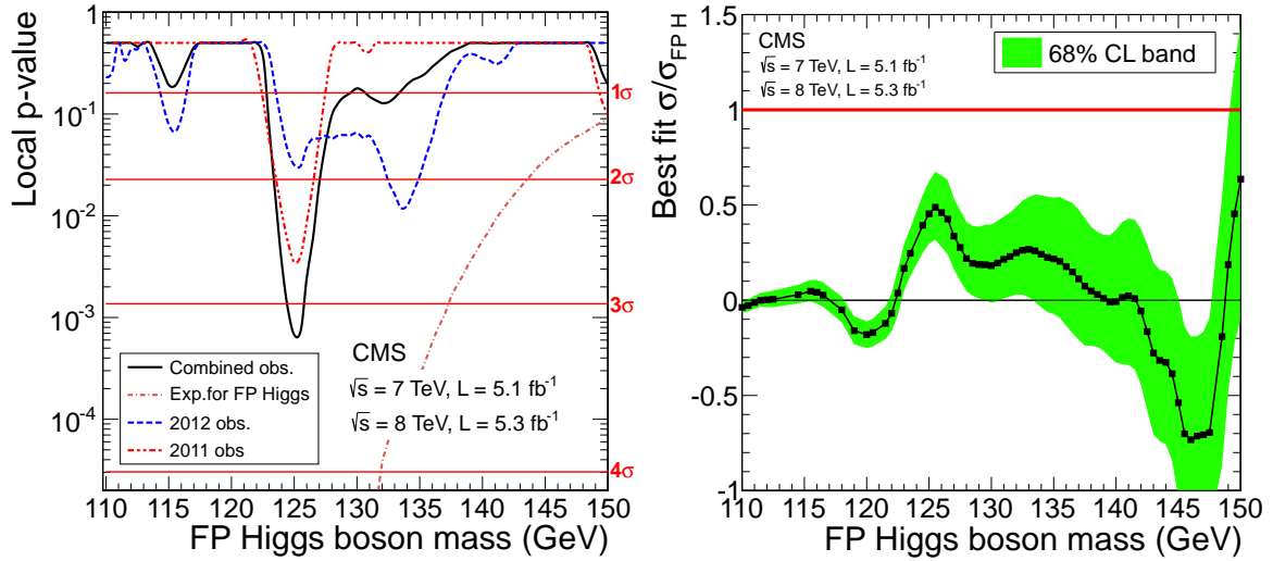
Figure 7: (left) The observed local p -value p_0 as a function of the FP Higgs boson mass in the range 110–150 GeV. The dashed-dotted line shows the expected local p -values should a fermiophobic Higgs boson with a mass m_H exist. The contributions to the expected limit for each run period are shown. (right) The best-fit \hat{\mu} = \sigma/\sigma_{\text{FPH}} as a function of the FP Higgs boson mass in the range 110–150 GeV. The band corresponds to the \pm 1 standard deviation uncertainty on the \hat{\mu} values.
