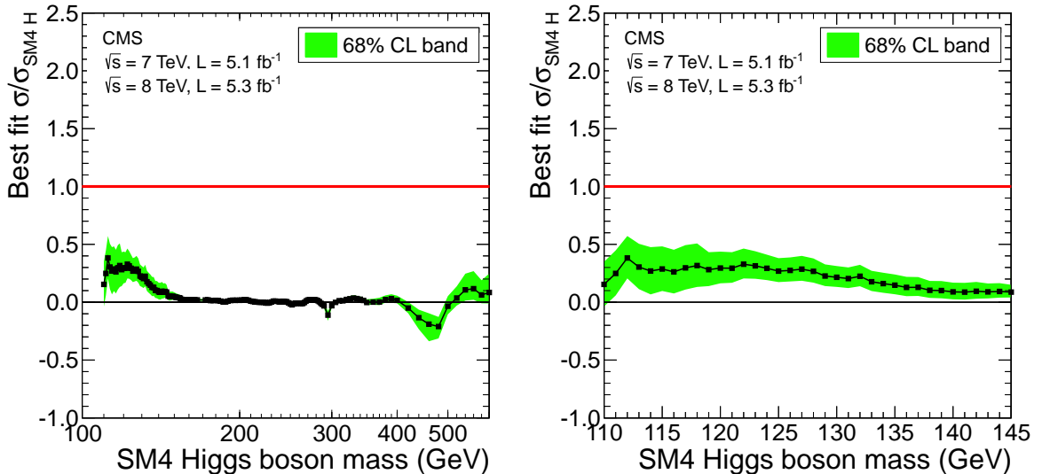
Figure 5: The best-fit \hat{\mu} = \sigma/\sigma_{\text{SM4H}} as a function of the SM4 Higgs boson mass in the range 110–600 GeV (left) and 110–145 GeV (right). The band corresponds to the \pm 1 standard deviation uncertainty on the \hat{\mu} values.
