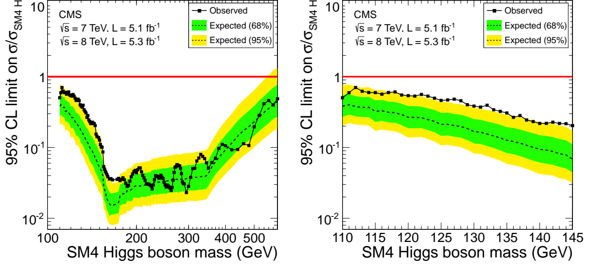
Figure 2: The observed and expected 95% CL upper limits on the signal strength modifier, \mu = \sigma/\sigma_{\text{SM4H}} , for the SM4 Higgs boson hypothesis as a function of the Higgs boson mass in the range 110–600 GeV (left) and 110–145 GeV (right).
