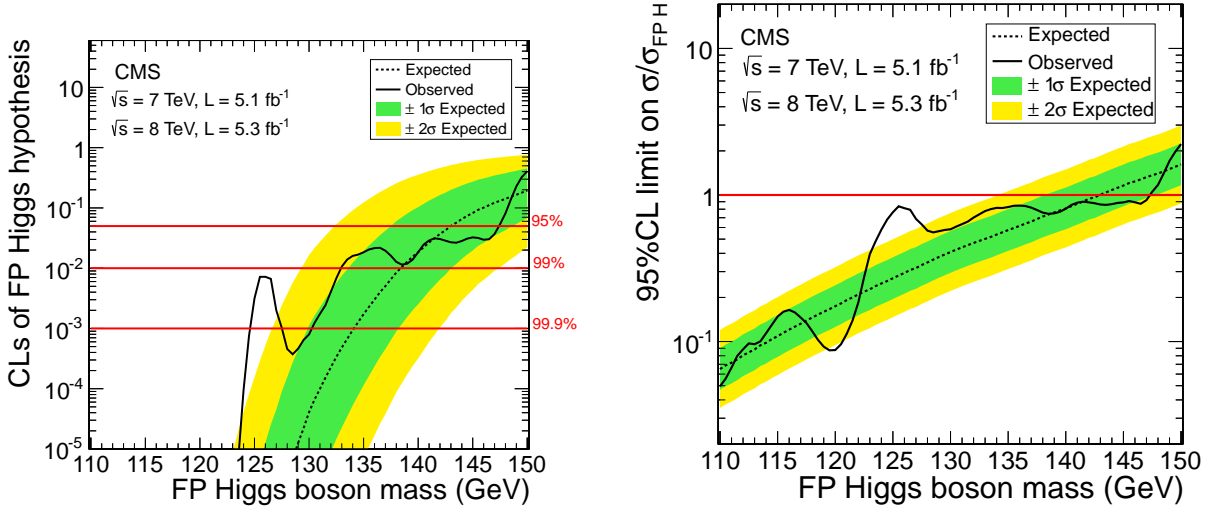
Figure 6: (left) The observed and expected CL_s values for the FP Higgs boson hypothesis as a function of the Higgs boson mass in the range 110–150 GeV. (right) The observed and expected 95% CL upper limits on the signal strength modifier, \mu = \sigma/\sigma_{\text{FP,H}} , as a function of the FP Higgs boson mass in the range 110–150 GeV.
