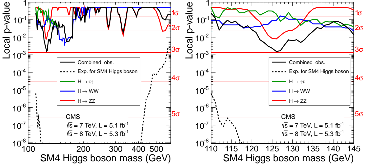
Figure 4: The observed local p_0 as a function of the SM4 Higgs boson mass in the range 110–600 GeV (left) and 110–145 GeV (right). The dashed line shows the expected local p -values should an SM4 Higgs boson with a mass m_H exist. The expected p -value is obtained with nuisance parameters constrained by the data, giving it some dependence on the observed data, and hence the small modulations on top of the overall smooth trend as a function of m_H .
