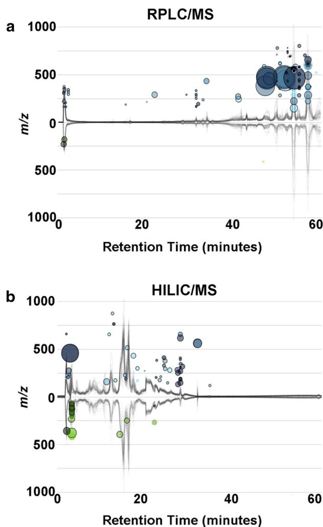
Fig. 2 Global liquid chromatography quadrupole time-of-flight mass spectrometry (LC-QTOFMS) metabolomics. Cloud plots generated by XCMS Online showing dysregulated features between control and PDR samples (two-tailed Mann–Whitney test) for a RPLC–MS analysis, control ( n = 11 ), PDR ( n = 9 ) top plot and b HILIC–MS analysis, control ( n = 11 ), PDR ( n = 7 ), lower plot. Total ion chromatograms (TICs) for each sample can be seen on the plot; features whose intensity are increased in PDR vitreous are shown on the upper part of the plot as blue circles and features whose intensity decreases are shown on the bottom part of the plot as green circles. Larger and brighter circles (features) correspond to larger fold changes and lower p -values respectively
