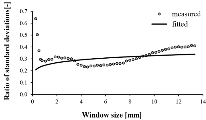
Figure 6. Ratio of \sigma_{total} / \sigma_{scanning} as a function of window sizes
