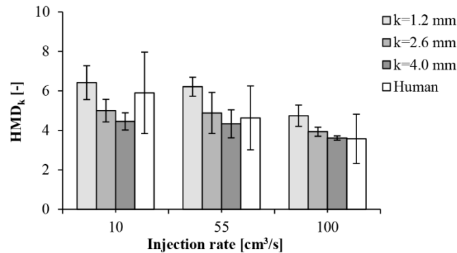
Figure 2. Inhomogeneity as a function of the injection molding rate and window size (k)
