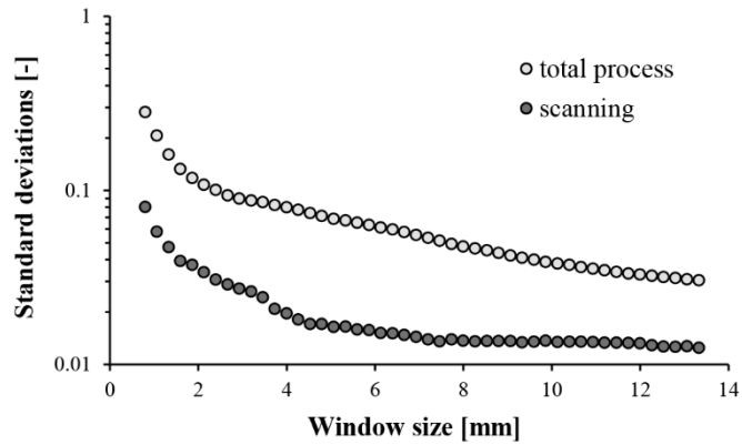
Figure 5. Normalized standard deviations of the scanning and the total process as a function of window sizes
