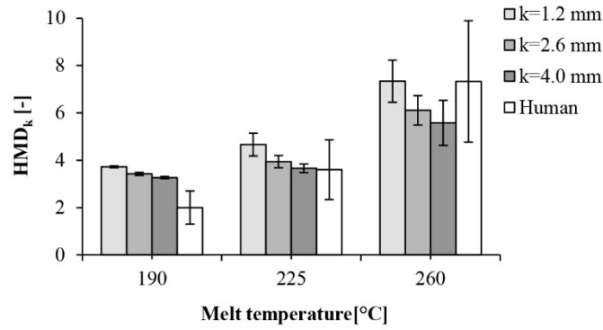
Figure 4. Inhomogeneity as a function of the melt temperature and window size (k)
