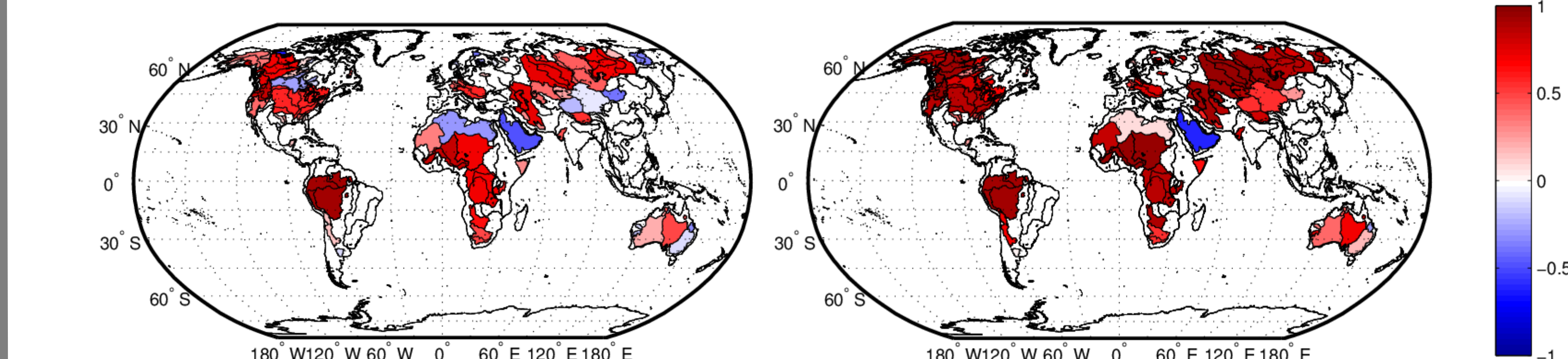
Figure 4: Correlation between storage mass changes derived from hydro-meteorological data and the combined solution (left) and GRACE GFZ Rel.05 (right)
