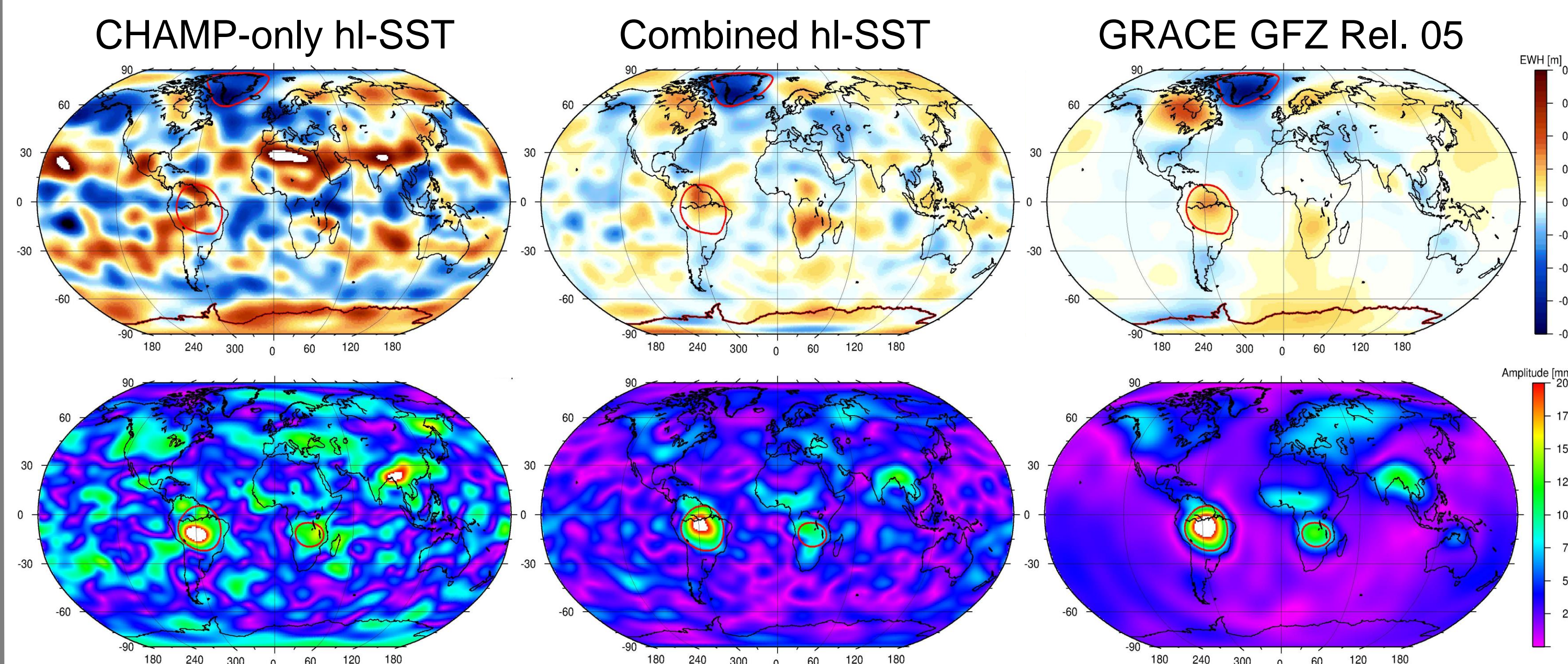
Figure 3: Trend (top) and annual amplitudes (bottom) of mass estimates derived from CHAMP-only (left), combined (middle) and the GRACE GFZ Rel. 05 (right) solution; Leakage out correction according to Baur et al. (2009) has been applied; Solutions have been filtered with a Gaussian 750km radius filter.
