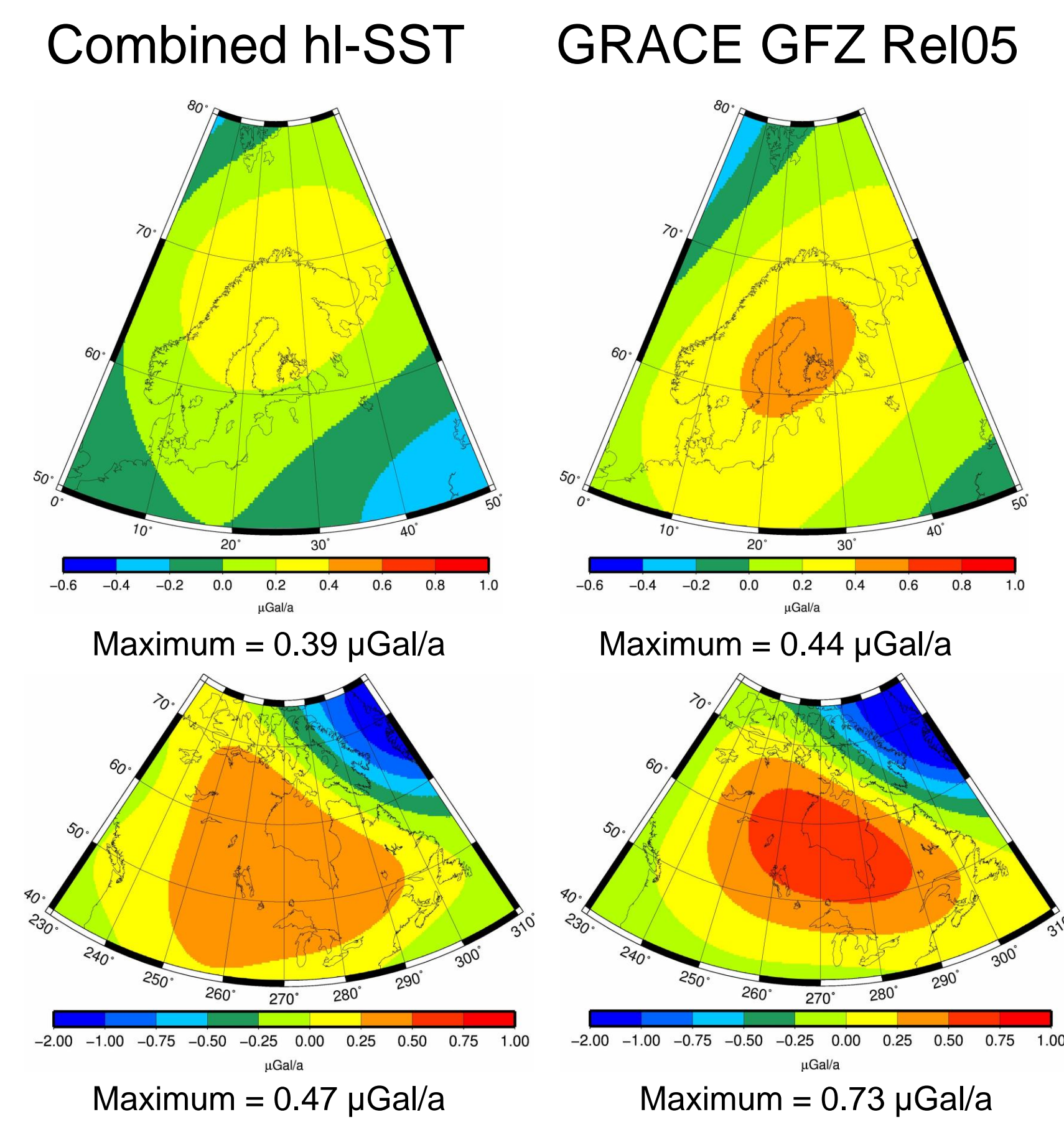
Figure 5: GIA pattern for the combined hl-SST solution (left) and for GRACE (GFZ, Rel. 05, right) for Scandinavia (top) and North America (bottom)
