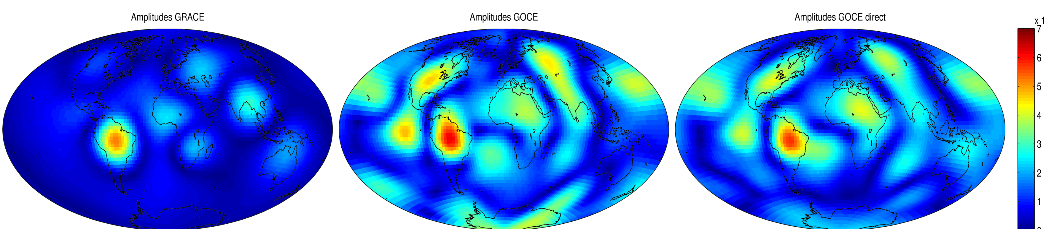
Figure 2: Amplitude in [mm] geoid height of the annual signal of GRACE (left), GOCE via monthly solution (middle) and GOCE via estimation (right); Gaussian smoothing with 1500km radius has been applied. Results available by contacting AIUB.
