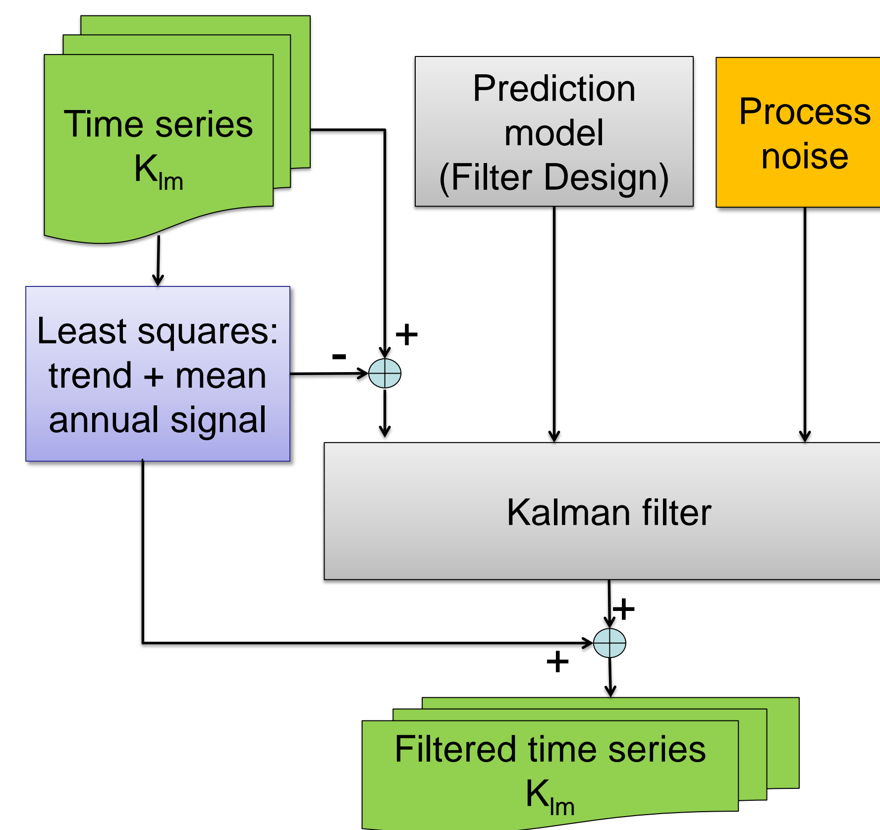
Figure 1: Scheme of the Kalman-Filtering
