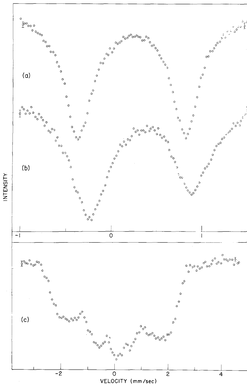
Figure 3. Mössbauer spectra of [\text{Fe}_4\text{S}_4(\text{SCH}_2\text{Ph})_4]^z at 77^\circ\text{K} : (a) z = 2^- in DMF; (b) z = 3^- in DMF/THF. (c) Spectrum of [\text{Fe}_4\text{S}_4(\text{SCH}_2\text{Ph})_4]^{3-} in DMF/THF at 4.2^\circ\text{K} with a longitudinal magnetic field of 1 kOe. Absorption lines at +0.7 and -0.4 mm/sec are due to residual dianion.
