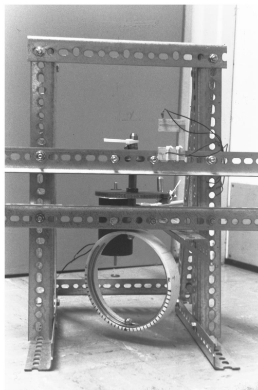
Fig. 2. Photograph of the bead on a hoop apparatus. The hoop is constructed from 6-in.-diam PVC pipe with brass rails on the interior to hold the steel ball. The hoop is suspended through two radial bearings using a half-inch diameter metal post and the post connected to the motor (visible at the back) by gears and a toothed plastic belt (available from Berg Manufacturing). Connected to the middle horizontal member is a photogate used to measure the rotation frequency. Power supply and frequency meter are not pictured.
