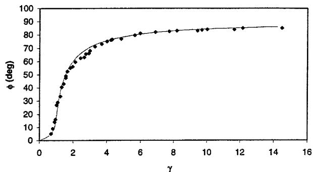
Fig. 3. Results from the bead on a hoop experiment (points). The solid line is a plot of a theoretically expected angular displacement ( \phi ) vs the parameter \gamma = r\omega^2/g for a hoop with the center of rotation slightly displaced from the radius of the hoop. r is the hoop radius, \omega is the angular velocity, and g the acceleration due to gravity. Note that the experimental data do not directly approach (0,0), showing a slight imperfection in the system.
