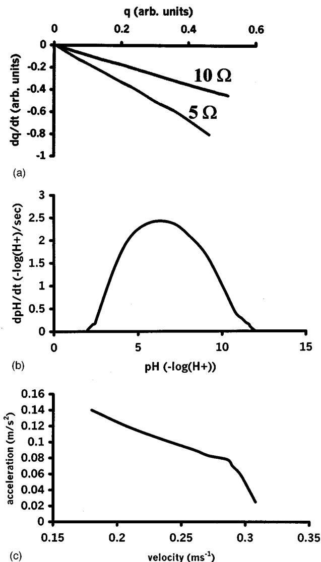
Fig. 1. Data from some simple one-dimensional systems experiments. (a) \dot{q} vs q in the RC experiment where the upper, line shows the result of using a 10\text{-}\Omega resistor and the lower line shows the result of a 5\text{-}\Omega resistor. (b) pH vs pH for the titration experiment. (c) \dot{v} vs v for the terminal velocity experiment. Note that cases (b) and (c) are nonlinear.
