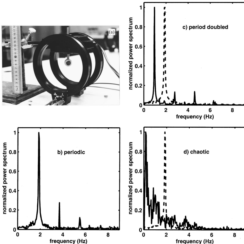
Fig. 5. (a) Photograph of the rotating magnet apparatus. (b), (c), and (d) show the result of the Fourier transform of the output when the motion is periodic, period doubled, and chaotic, respectively (solid curves). The dotted curves show the power spectrum of the driver at 1.8 Hz.
