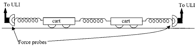
Fig. 4. Schematic of the coupled oscillator experiment.
