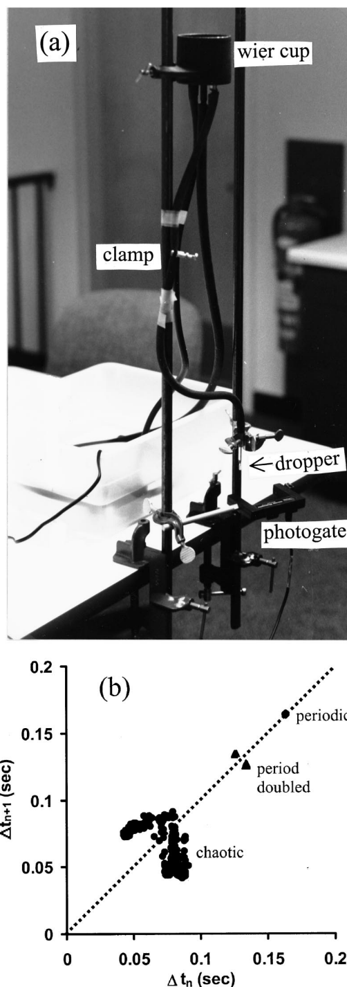
Fig. 6. (a) Photograph of the dripping faucet apparatus. (b) Return maps generated from the dripping faucet experiment showing, at different flow rates, the appearance of periodic, period doubled, and chaotic behavior.
