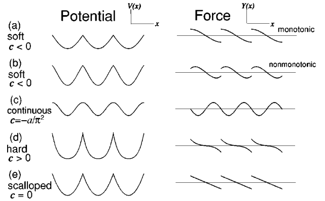
FIG. 1. Sketches of the pinning potentials and forces studied in this paper. The pinning forces are periodic with period 2\pi and the pinning potential for a degree of freedom \theta_i has minima at \beta_i + 2n\pi , for integer n . The cases are organized primarily by the sign of c , with the pinning force Y(x) = -ax - cx^3 + O(x^5) for small x = \theta_i - \beta_i . The coefficient of the harmonic part of the force satisfies a > 0 . The cases (a), (b) and (c) are for “soft” pinning forces ( c < 0 ); they differ near the potential maxima, corresponding to monotonic, non-monotonic, and continuous forces, respectively. Case (d) is a “hard” potential ( c > 0 ). The “scalloped” potential, case (e), is precisely quadratic ( c = 0 ) in the interval -\pi < x < \pi . The form of the potential especially affects the stability of the coherently pinned phase and whether “re-entrant” pinning is possible upon increasing or decreasing the force.
