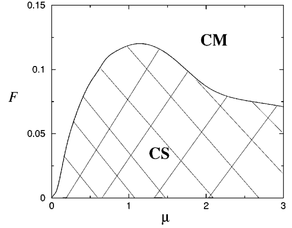
FIG. 20. Phase diagram in the \mu - F plane for a piecewise linear pinning force, with a=1/\pi and c=0 , and \rho(h)=e^{-h} . The depinning curve has been obtained numerically for a system with N=1024 and a ramp rate of dF/dt=10^{-6} .
