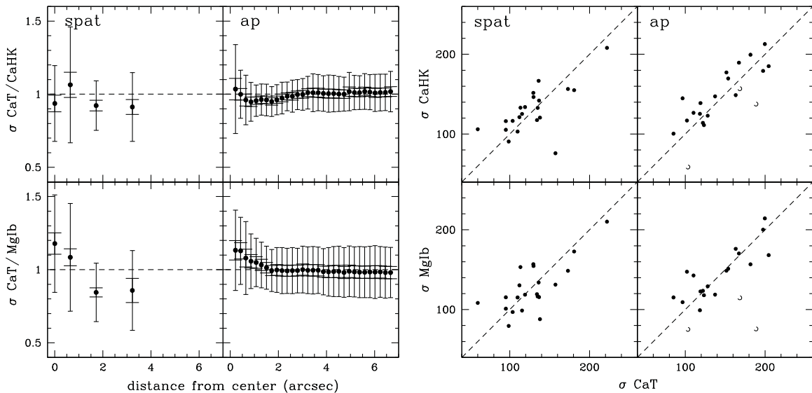
Figure 15. Comparison of stellar-velocity dispersion as measured from CaT, CaHK, and MgIb region. (a) Ratio of stellar-velocity dispersions measured from CaT to MgIb (lower panels) and CaHK (upper panels) as a function of distance from the center. The mean is shown at each location including the rms error (shorter—in x —horizontal bar) and the error on the mean (longer—in x —horizontal bar). Note that the rms scatter is due to both intrinsic scatter and measurement errors which contribute at the level of 7%–15%. The dashed line corresponds to a ratio of 1. From spatially resolved spectroscopy in the left panels ( \sigma_{\text{spat}} ; i.e., the centroid of the extracted spectra from which the ratio was measured is at the distance from center that is indicated on the x -axis with aperture sizes as discussed in Section 4.1 and with the measurement on both sides of the nucleus averaged); from aperture spectra in the right panels ( \sigma_{\text{ap}} ; i.e., the spectra from which the ratio was measured are always centered on the nucleus but the width of the extracted aperture increases as indicated on the x -axis). (b) One-to-one comparison for the luminosity-weighted stellar-velocity dispersion within the effective radius: CaT vs. MgIb (lower panels) and CaT vs. CaHK (upper panels) for spatially resolved spectra in the left panels ( \sigma_{\text{spat,ref}} ) and for aperture spectra ( \sigma_{\text{ap,ref}} ) in the right panels, respectively. The open symbols in the left panels indicate three outliers that were excluded in panel (a).
