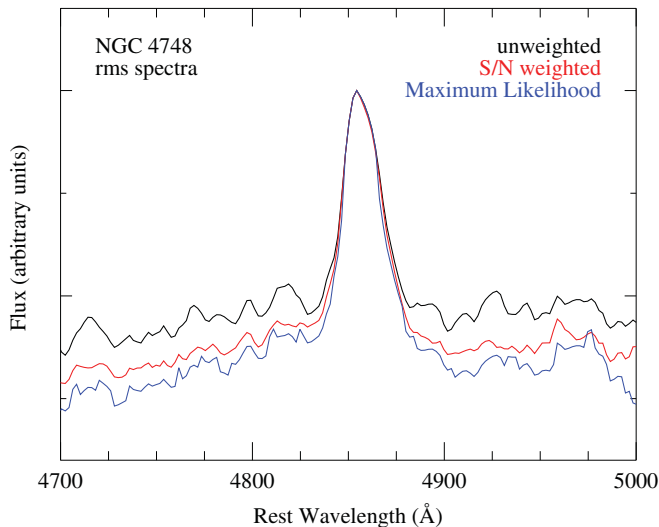
Figure 3. Comparison of the rms spectra of NGC 4748 generated with three different methods: unweighted rms (black), S/N weighted (red), and maximum likelihood (blue). For this object, two bad epochs with low-S/N data were removed as described in Section 3.2.
