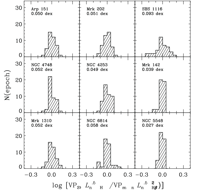
Figure 12. Distribution of the SE virial product ( V^2 \times L^{0.5} ) normalized to that of the mean spectra. H\beta line dispersion is used for the velocity and the nuclear luminosity at 5100 \text{ \AA} , corrected for the host galaxy, is used for the luminosity. The average rms dispersion of all nine objects is 0.052 \pm 0.006 dex.
