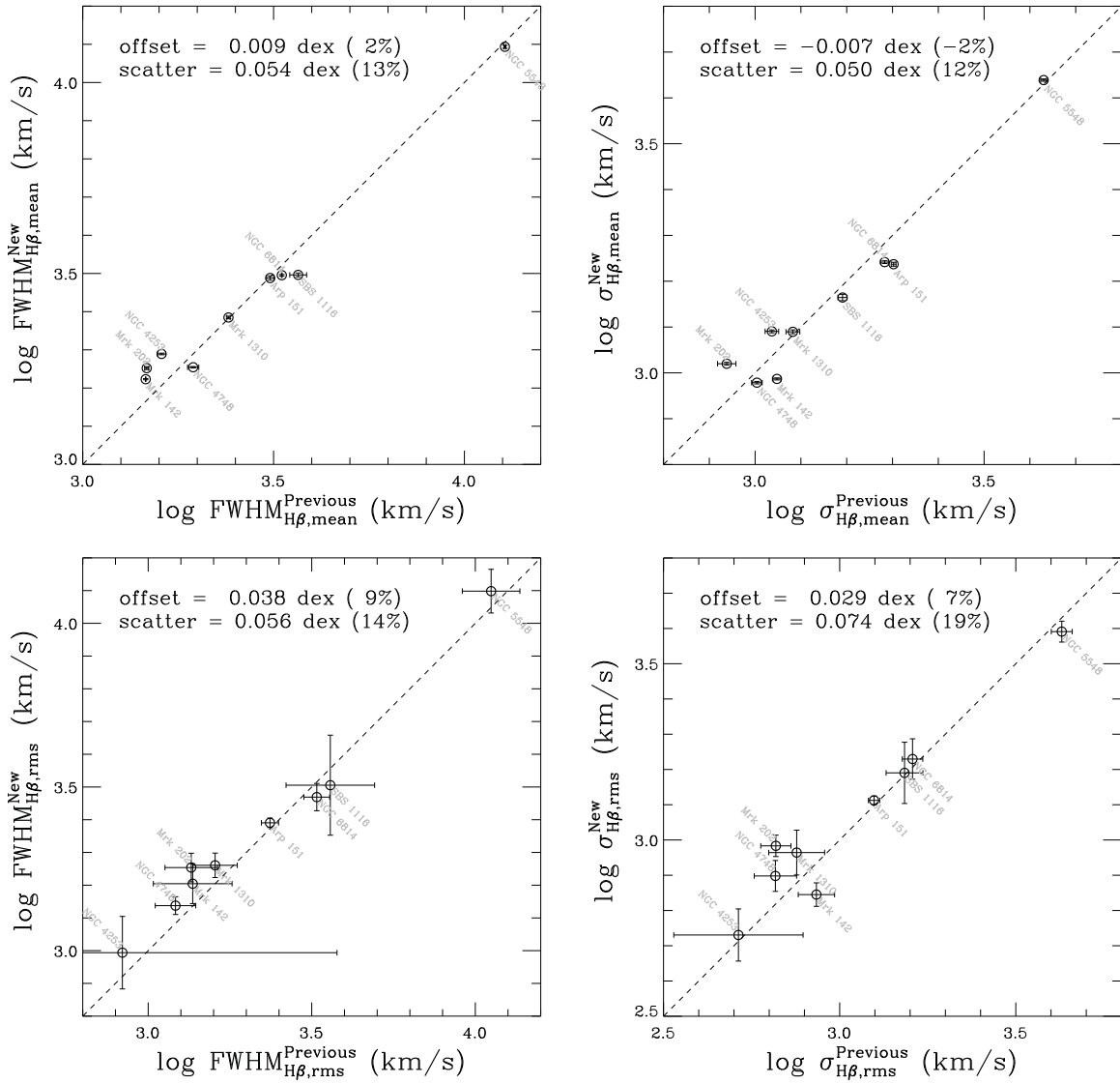
Figure 17. Comparison of FWHM Hβ (left) and σ Hβ measurements (right) based on the new methods (this work) and the previous traditional methods (Bentz et al. 2009c), using the mean (top) and rms spectra (bottom). The average difference of the Hβ line widths between two methods is relatively small. However, the large scatter (12%–19%) indicates that the contribution from individual effects, e.g., subtraction of starlight, Fe II or He II, varies on an object-by-object basis.
