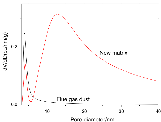
Fig. 3 Pore size distributions of flue gas dust and new matrix prepared at \text{Na}_2\text{O}/\text{Al}_2\text{O}_3 ratio of 6.0
