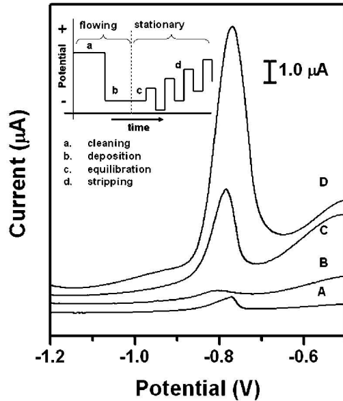
Fig. 4 Square-wave anodic stripping voltammograms for 25 ppb solution of Pb(II) in 0.1 M acetate buffer (pH 4.5) in the presence of 25 ppb Zn(II) : (A) a 100 µL solution placed directly on the electrodes; (B) a 100 µL solution added to the stagnant µPEDs (without a pad of blotting paper as sink); (C and D) a solution of analytes continuously wicking the paper channel of the hydrodynamic µPEDs. The deposition time was 120 s (A, B, C) or 360 s (D). The SWASV was performed in the potential range of -1.2 to -0.5 V under optimized conditions: frequency, 20 Hz; amplitude, 25 mV; potential increment, 5 mV; equilibration time, 30 s. Deposition was performed at -1.2 V; 'cleaning' was performed at +0.5 V for 60 s. A bismuth(III) concentration of 500 µg L -1 was chosen for the co-deposition of heavy-metal ions. We used screen-printed carbon electrodes as the working and counter electrodes, and a screen-printed Ag/AgCl electrode as the reference electrode. Inset shows the schematic of the four steps of the square-wave anodic stripping voltammetry.
