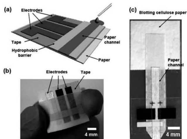
Fig. 1 (a) Schematic of a paper-based electrochemical sensing device. The sensor comprises three electrodes printed on a piece of paper substrate (or plastic) and a paper channel. The paper channel was in conformal contact with the electrodes, and was held in place by double-sided adhesive tape surrounding the electrodes. A photograph of a paper-based electrochemical sensing device for the analysis of glucose (b), and a hydrodynamic paper-based electrochemical sensing device for the measurement of heavy-metal ions (c). The device consists of two printed carbon electrodes as the working and counter electrodes, and a printed Ag/AgCl electrode as the pseudo-reference electrode. The paper channel was fabricated by patterning SU-8 as a hydrophobic barrier for aqueous solution. The paper channel in (b) was colored with red ink to enhance imaging. The dashed line in (c) indicates the edge of the paper channel. The scale bar is 4 mm.
