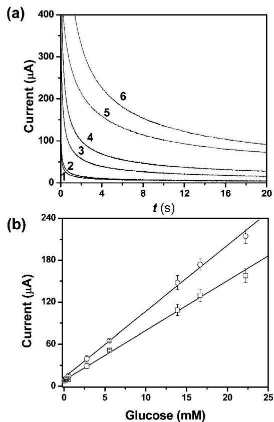
Fig. 3 (a) Representative chronoamperometric curves for glucose concentrations (mM): 0 (1), 0.2 (2), 2.8 (3), 5.6 (4), 13.9 (5) and 22.2 (6) in the \mu PEDs. (b) Calibration plots of current as a function of the concentration of glucose for the detection of glucose in the \mu PEDs ( \square ) and in bulk solutions ( \circ ). We used three carbon electrodes as working, counter, and pseudo-reference electrodes, respectively. The working electrodes had a surface area of 16 \text{ mm}^2 in contact with the solution in both the \mu PEDs and the bulk solutions. The distance between electrodes was 1.0 mm. A 500 mV step potential (vs. a carbon pseudo-reference electrode) was used to generate the calibration curve. The solid line represents a linear fit to ( \square ) with regression equation: y = 9.5 + 6.9x ( R^2 = 0.995 , n = 8 ), and a linear fit to ( \circ ) with regression equation: y = 12.1 + 9.4x ( R^2 = 0.997 , n = 8 ).
