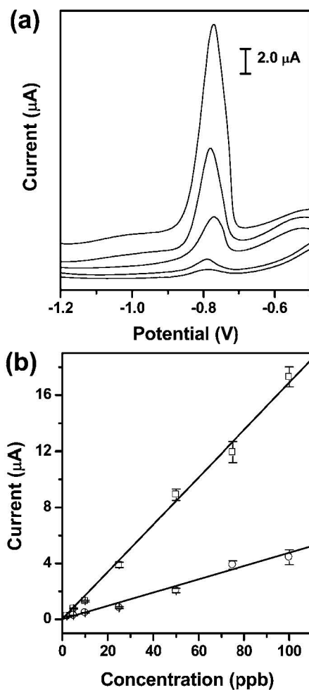
Fig. 5 (a) Square-wave anodic stripping voltammograms for the analysis of trace \text{Pb(II)} in 0.1 M acetate buffer (pH 4.5) in the presence of \text{Zn(II)} (1: 1 molar ratio of \text{Pb(II)} to \text{Zn(II)} ) in the \mu\text{PEDs} with a solution of analytes continuously wicking along the paper channel. The concentrations (ppb) of \text{Pb(II)} (ascending along the y-axis) are 5, 10, 25, 50, and 100. The data are unsmoothed. (b) The resulting calibration plots for the analysis of trace \text{Pb(II)} : a 100 \mu\text{L} solution of analytes placed on the electrodes (○), and a solution of analytes continuously wicking along the paper channel in the \mu\text{PEDs} (□). Square-wave voltammetric stripping was performed in the potential range of -1.2 to -0.5 V under optimized conditions: frequency, 20 Hz; amplitude, 25 mV; potential increment, 5 mV; equilibration time, 30 s. Deposition was performed at -1.2 V for 120 s; ‘cleaning’ was performed at +0.5 V for 60 s. A bismuth(III) concentration of 500 \mu\text{g L}^{-1} was chosen for the co-deposition of heavy-metal ions. We used screen-printed carbon electrodes as working and counter electrodes, and a screen-printed Ag/AgCl electrode as the reference. The solid lines represent a linear fit to (○) with regression equation: y = -0.08 + 0.05x ( R^2 = 0.978 , n = 8 ), and a linear fit to (□) with regression equation: y = -0.21 + 0.17x ( R^2 = 0.996 , n = 8 ).
