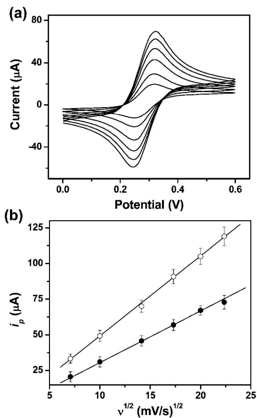
Fig. 2 (a) Cyclic voltammograms of 2.0 mM ferrocene carboxylic acid in 0.5 M KCl aqueous solution (pH = 7.0) in a \mu PED at various scan rates (ascending along y-axis): 50, 100, 200, 300, 400, and 500 \text{mV s}^{-1} . We used a 4 mm by 4 mm carbon-printed electrode as the working electrode, and a printed Ag/AgCl electrode as the reference electrode. (b) The plot of anodic peak current vs. the square root of the scan rate ( v^{1/2} ) for CV experiments conducted on a paper device (●) and in a bulk solution (○). The solid lines represent a linear fit to (●) with regression equation: y = -3.6 + 3.5x ( R^2 = 0.998 , n = 8 ), and a linear fit to (○) with regression equation: y = -7.1 + 5.6x ( R^2 = 0.999 , n = 8 ).
