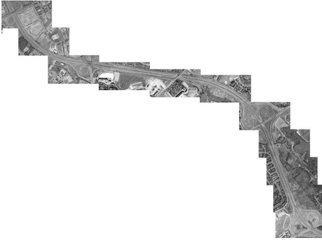
Fig. 9. The Vissim traffic network used for testing the GPS coordinate following routine
