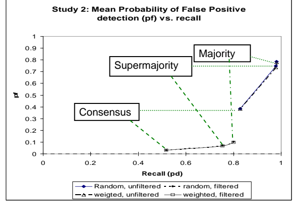
Figure 9. Study 2: Mean probability of false positive detection ( pf ) vs. probability of detection (recall).
