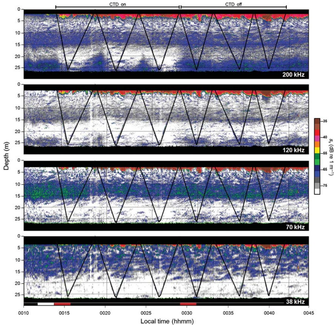
Fig. 1. Sample echograms at four frequencies overlaid with the depth profiles of six CTD casts, three normal and three with the CTD powered off. Acoustic volume backscattering in dB is shown in color with white representing scattering below threshold. The strong scattering near the surface is from air bubbles entrained by the boat's hull. Noticeable decreases in acoustic scattering a few meters above the seafloor (shown in black) can be seen in the 200 kHz echogram (top panel) with somewhat weaker decreases midwater can be seen when the CTD was powered on, but no avoidance is detectable when the CTD was not powered indicating that the avoidance was not caused by the physical movement of the profiling package. Avoidance is less apparent at 120 kHz and undetectable at lower frequencies. The 2-min time interval integrated to provide a background estimate of acoustic scattering is indicated by a white bar near the time axis, while the acoustic integration intervals during the first cast of each profile set are indicated by red bars.
