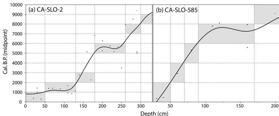
Fig. 2. Component definitions for (a) CA-SLO-2 and (b) CA-SLO-585 based on the relationship between depth (cm) and BP * midpoint. Fitted spline ( \lambda = 10,000 ) describes the relationship between depth and calibrated years BP. Components appear in shaded grey.
