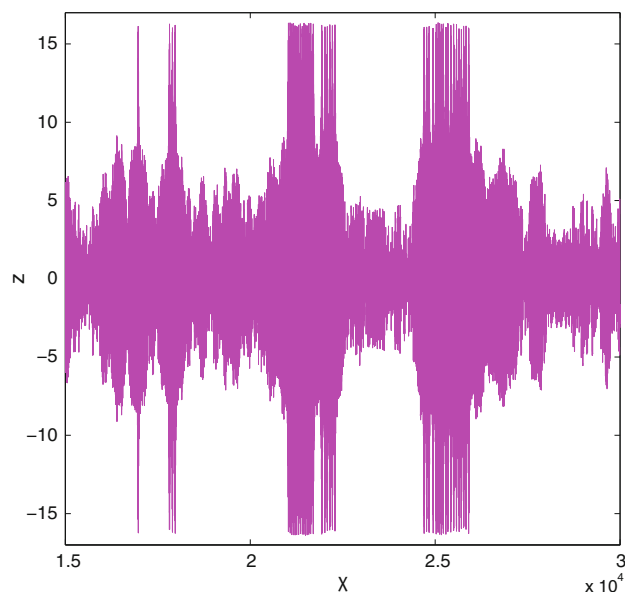
Fig. 10 Chaotic motions of Z based on system (24)
